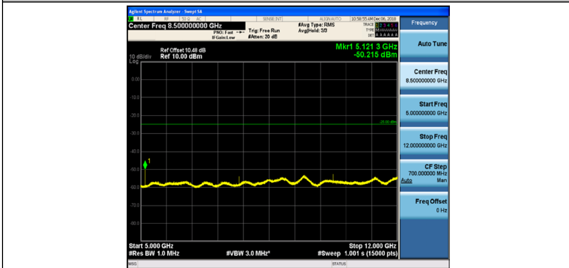
Band7_10MHz_16QAM_21400_1RB#0
