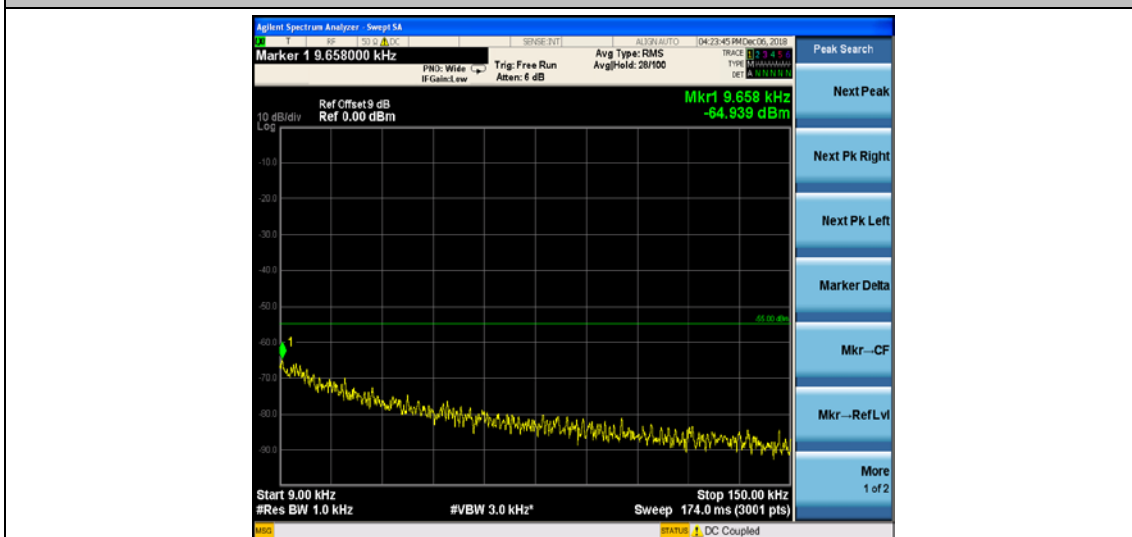
Band7_15MHz_16QAM_21100_1RB#0
