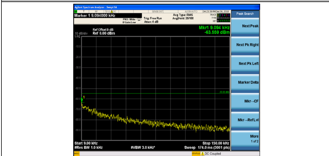
Band7_15MHz_16QAM_20825_1RB#0
