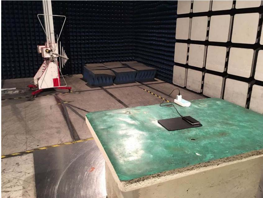
Photos of Radiation Emission Measurement
