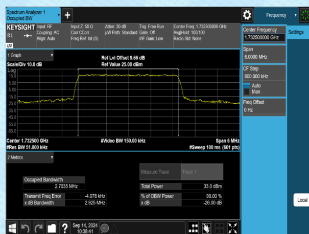
Band4-3MHz-16QAM-20175-15RB#0-PASS
