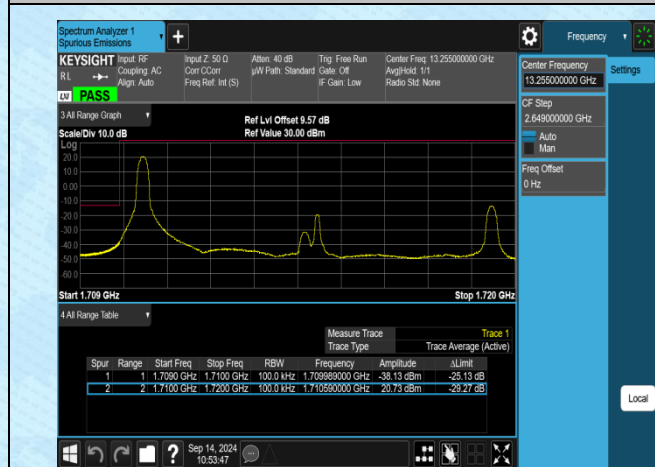
Band4-10MHz-16QAM-20000-1RB#0-PASS
