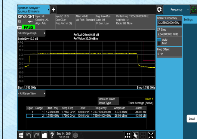
Band4-10MHz-QPSK-20350-50RB#0-PASS
