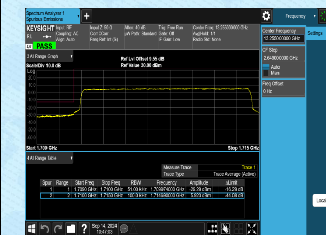
Band4-5MHz-QPSK-19975-25RB#0-PASS
