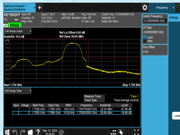
Band4-1.4MHz-16QAM-20393-1RB#5-PASS
