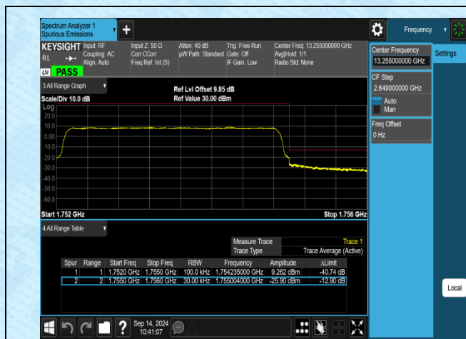
Band4-3MHz-QPSK-20385-15RB#0-PASS
