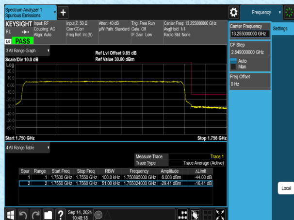
Band4-5MHz-16OAM-20375-25RB#0-PASS
