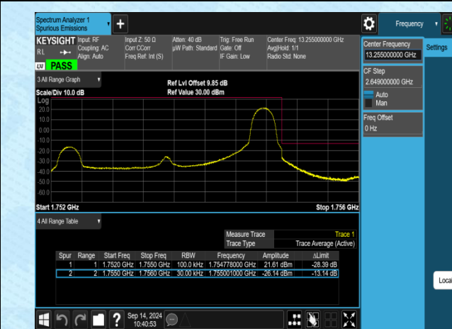
Band4-3MHz-16QAM-20385-1RB#14-PASS
