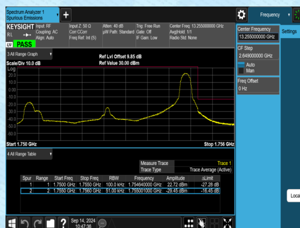
Band4-5MHz-QPSK-20375-1RB#24-PASS
