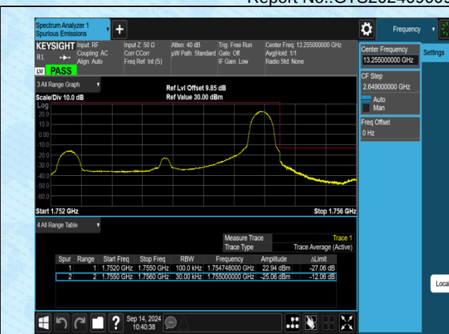
Band4-3MHz-QPSK-20385-1RB#14-PASS
