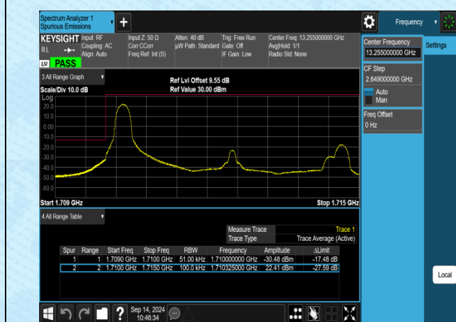
Band4-5MHz-QPSK-19975-1RB#0-PASS
