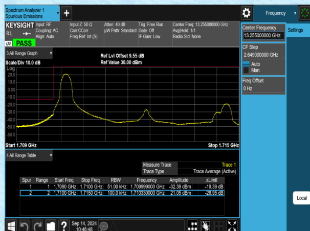
Band4-5MHz-16OAM-19975-1RB#0-PASS
