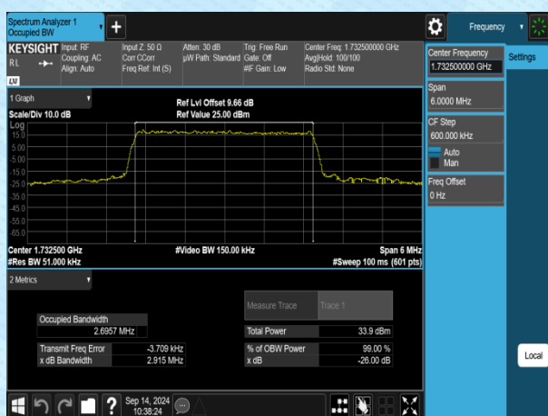
Band4-3MHz-QPSK-20175-15RB#0-PASS
