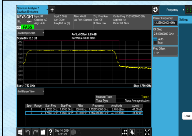
Band4-3MHz-16QAM-20385-15RB#0-PASS
