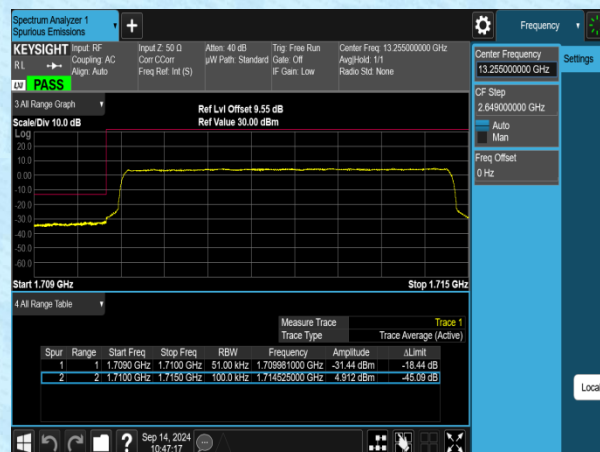
Band4-5MHz-16OAM-19975-25RB#0-PASS
