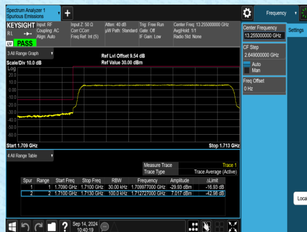
Band4-3MHz-16OAM-19965-15RB#0-PASS
