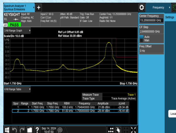
Band4-5MHz-16OAM-20375-1RB#24-PASS
