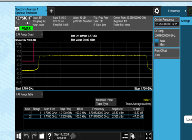
Band4-10MHz-16QAM-20000-50RB#0-PASS
