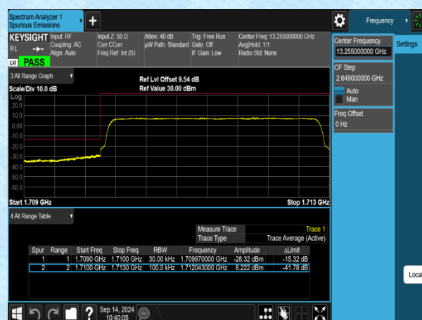
Band4-3MHz-QPSK-19965-15RB#0-PASS
