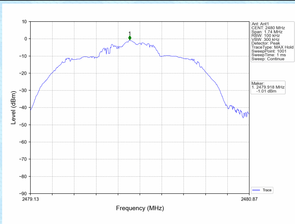
\pi/4 -DQPSK_2DH5_HCH_2480MHz_Ant1_NTNV
