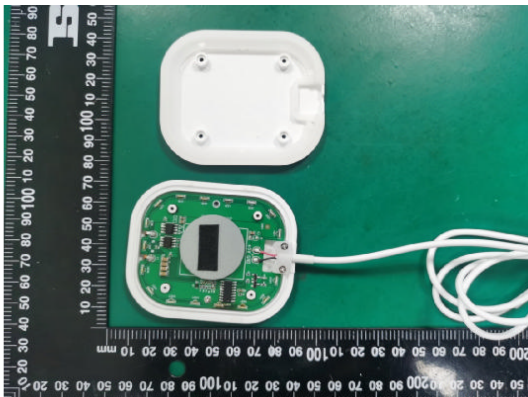
Internal Photo FCC ID: 2AR4R-QAP10
