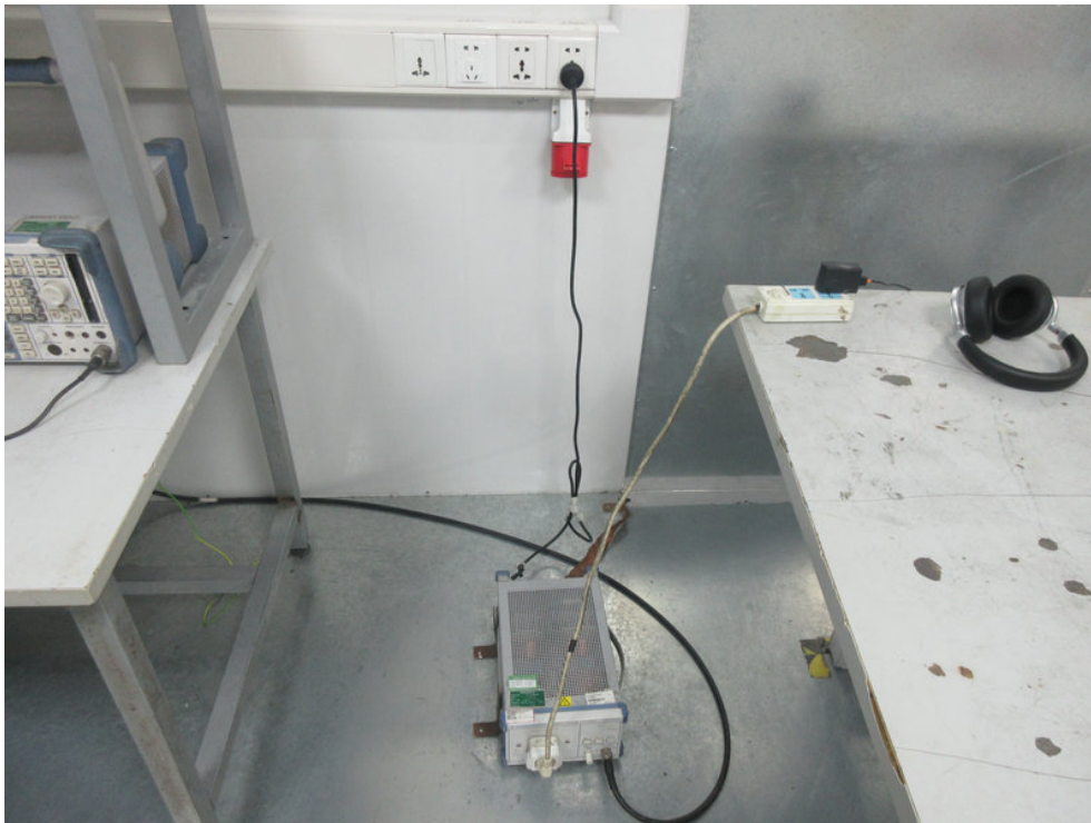
FCC ID: 2AR52-H1010 Photo of Conducted Emission Measurement
