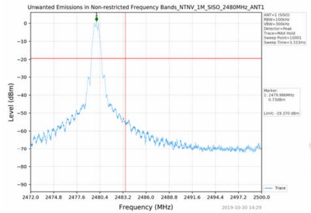
Right bandedge
