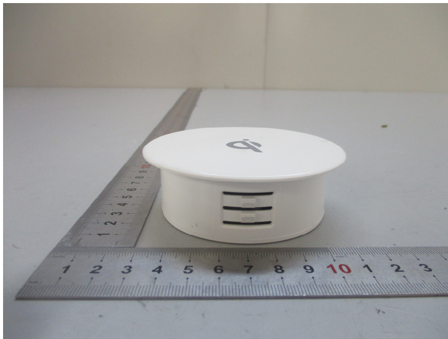
EUT(DOCK-950-B-QC-BK)– Front View
