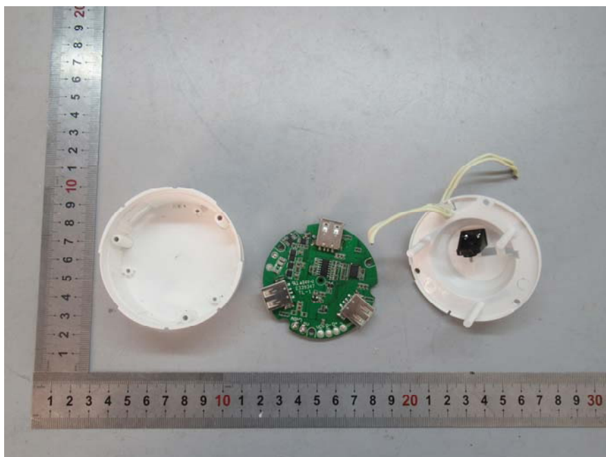
EUT(DOCK-150-B-BK) – Cover off View-4
