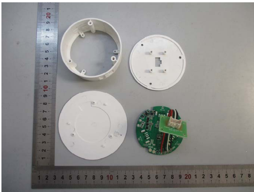
EUT (DOCK-950-B-QC-BK) – Cover off View
