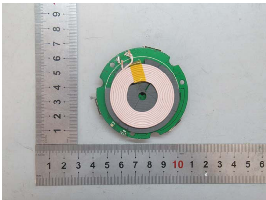
EUT(DOCK-150-B-BK) – PCB2 Bottom View
