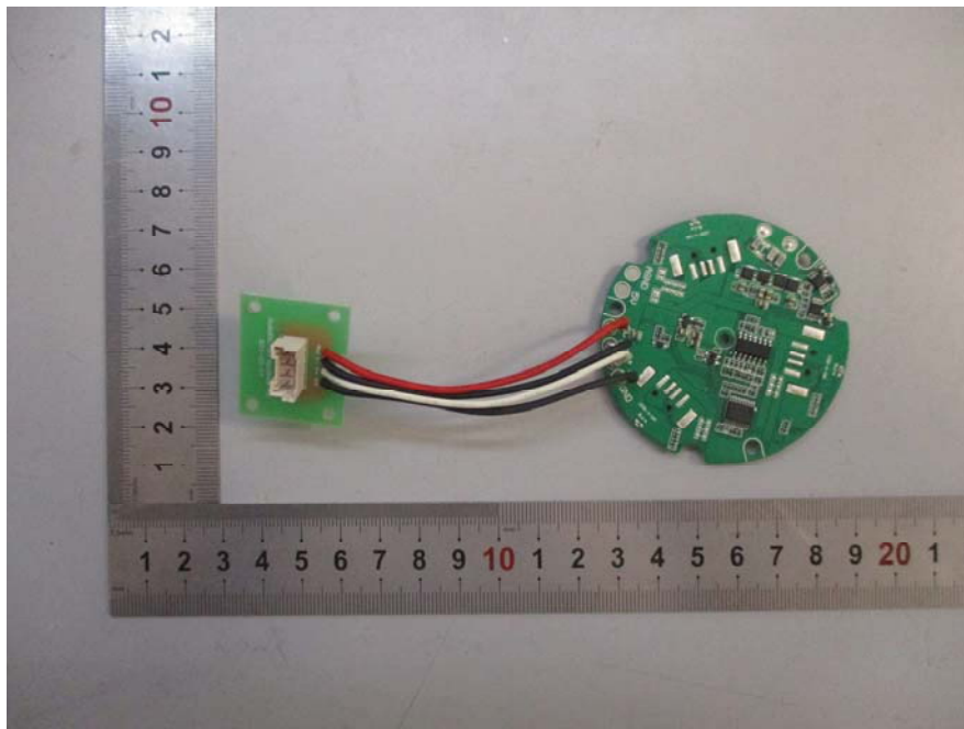
EUT(DOCK-950-B-QC-BK) – PCB Bottom View
