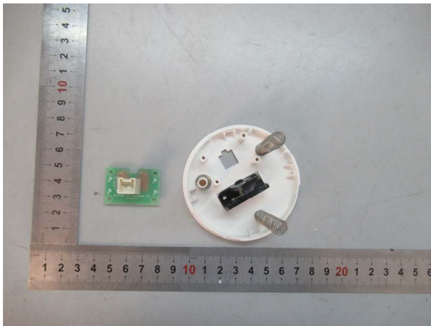
EUT(DOCK-150-B-BK) – Cover off View-2
