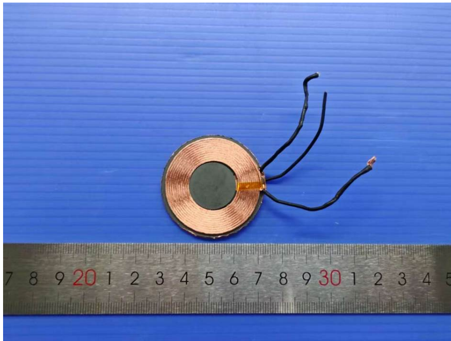
WPT Coil
