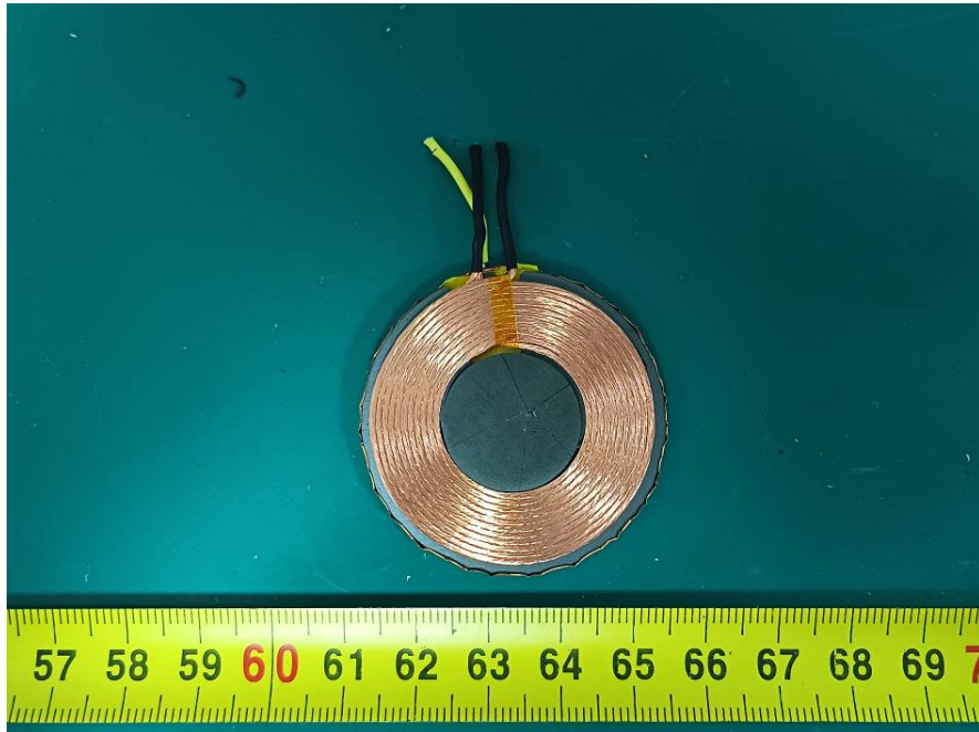
WPT Coil
