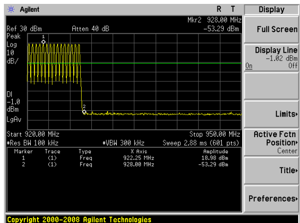
ASK: Band Edge-High Channel (Hopping Mode)
