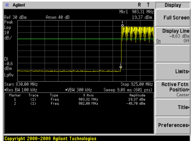
ASK: Band Edge-High Channel
