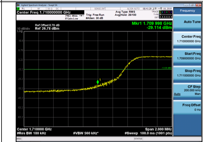
LCH_16QAM_50RB#0
