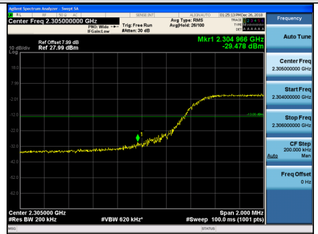
LCH_16QAM_50RB#0
