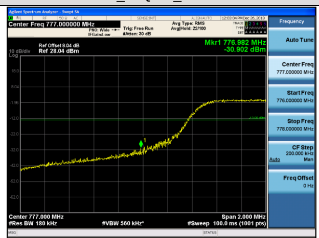
LCH_16QAM_50RB#0
