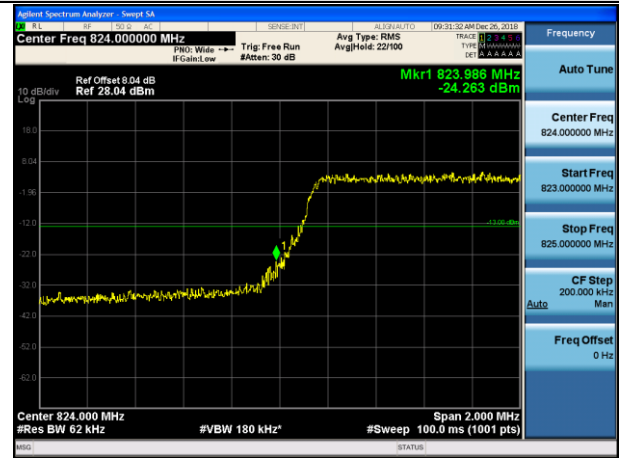
LCH_16QAM_15RB#0
