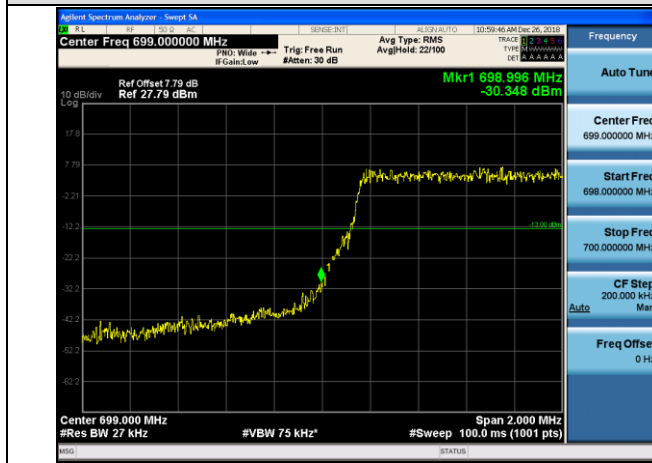
LCH_QPSK_6RB#0
