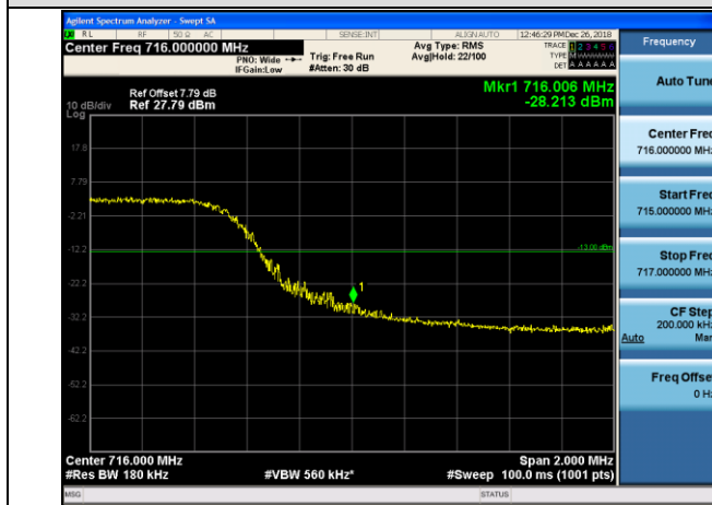
HCH_QPSK_50RB#0
