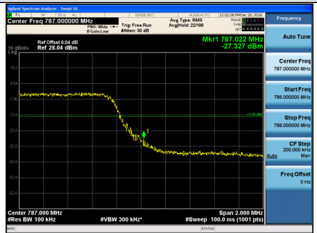
HCH_16QAM_25RB#0
