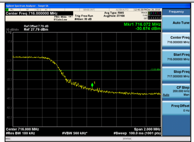
HCH_16QAM_50RB#0
