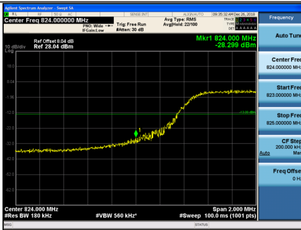
LCH_QPSK_50RB#0
