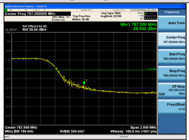
HCH_16QAM_50RB#0
