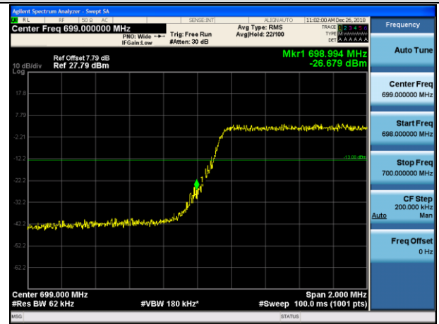
LCH_16QAM_15RB#0
