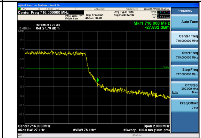
HCH_16QAM_6RB#0
