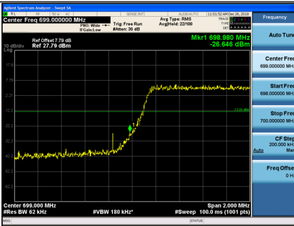
LCH_QPSK_15RB#0
