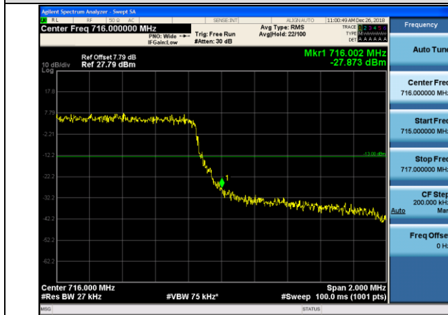
HCH_QPSK_6RB#0
