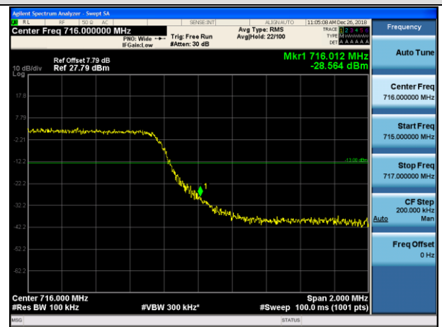
HCH_16QAM_25RB#0
