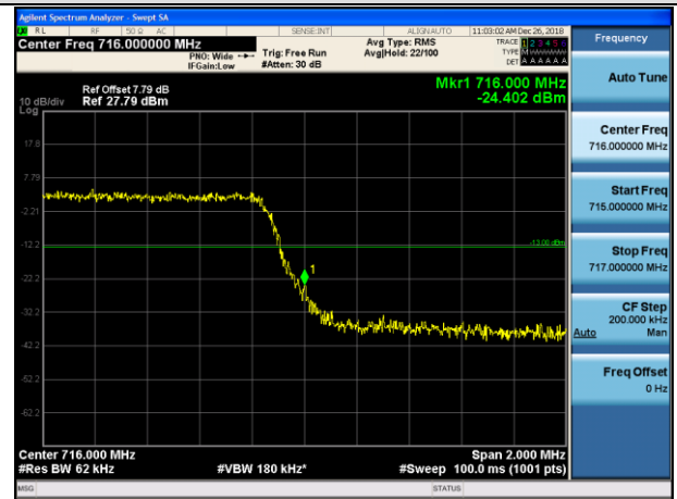
HCH_16QAM_15RB#0
