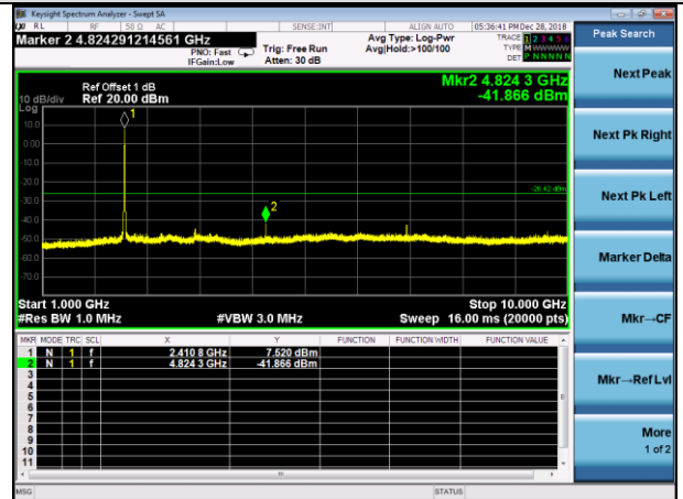
11B-LCH
