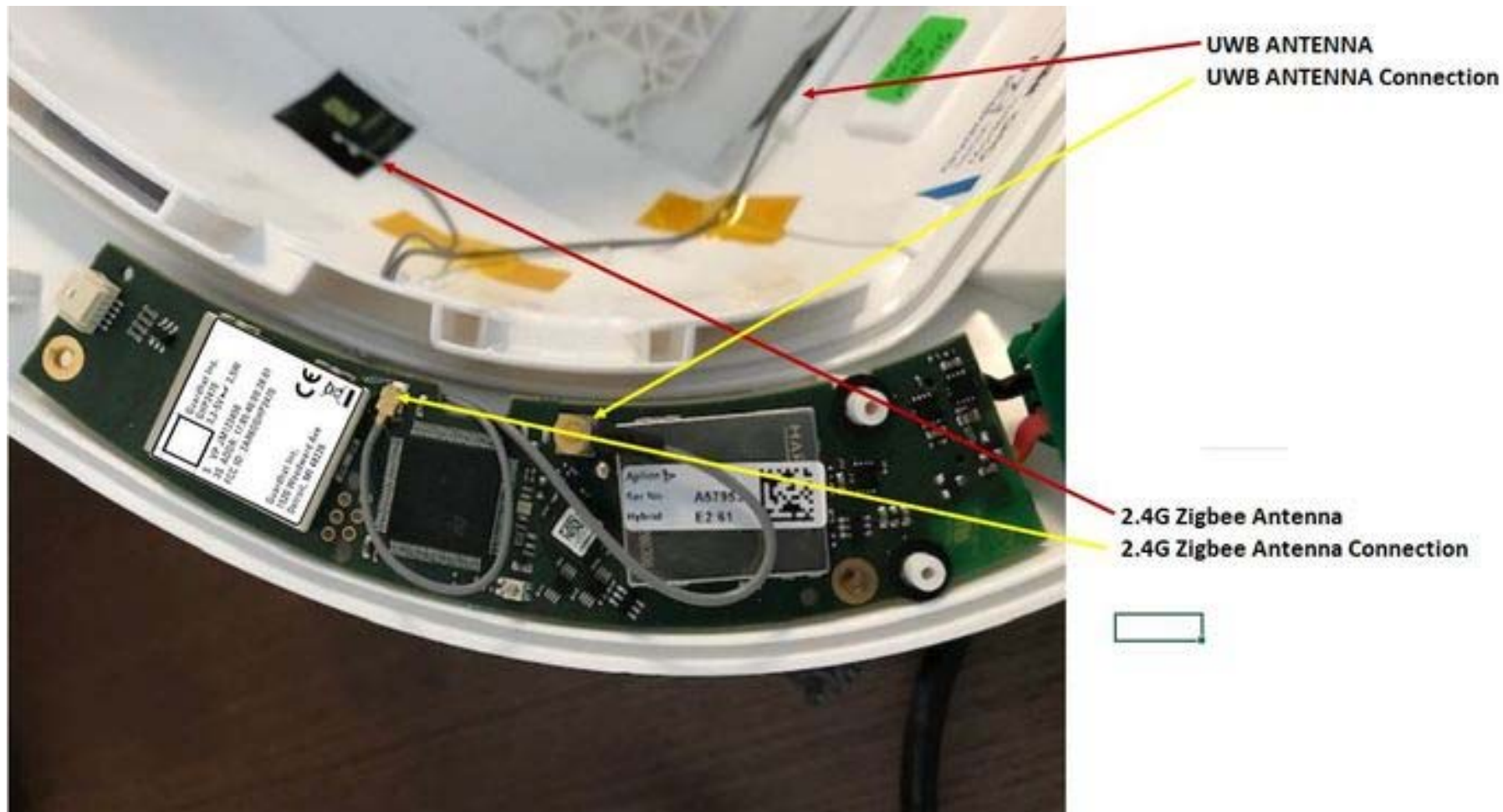
Position board Antenna Connections UWB and Zigbee
