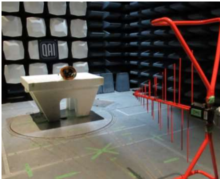
Figure 2: Radiated Emissions (30 MHz – 1 GHz) performed at the SAC Test Setup
