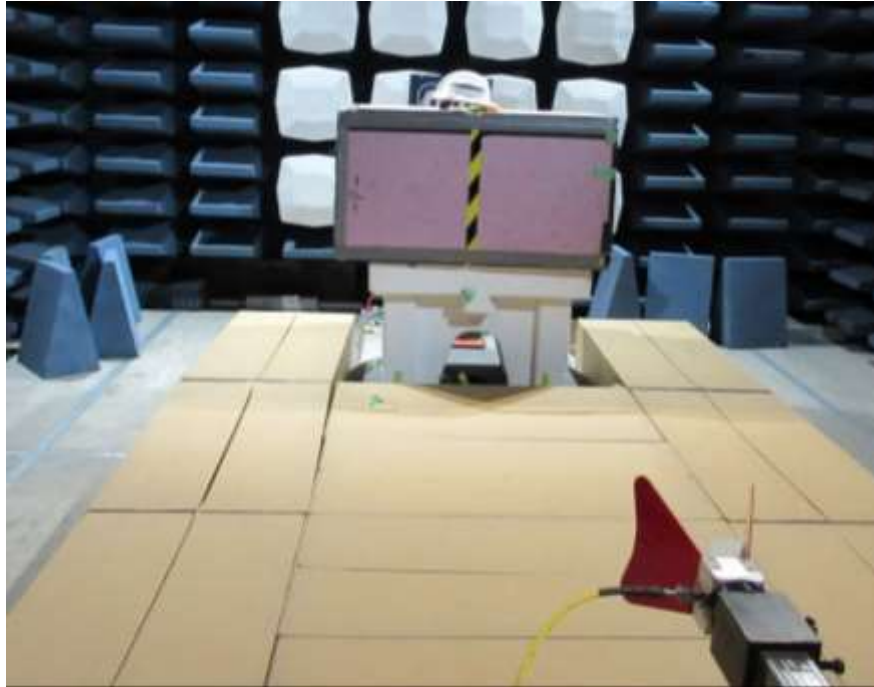
Figure 3: Radiated Emissions (1 – 13 GHz) performed at the SAC Test Setup
