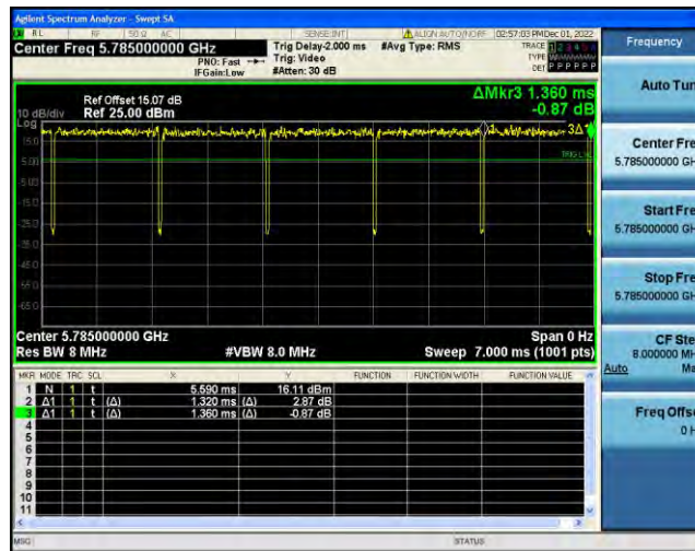
NTNV-11AC20SISO-Ant2-5785-1.32-1.36
