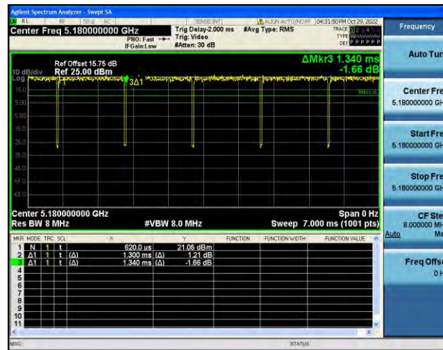
NTNV-11N20SISO-Ant2-5180-1.31-1.35
