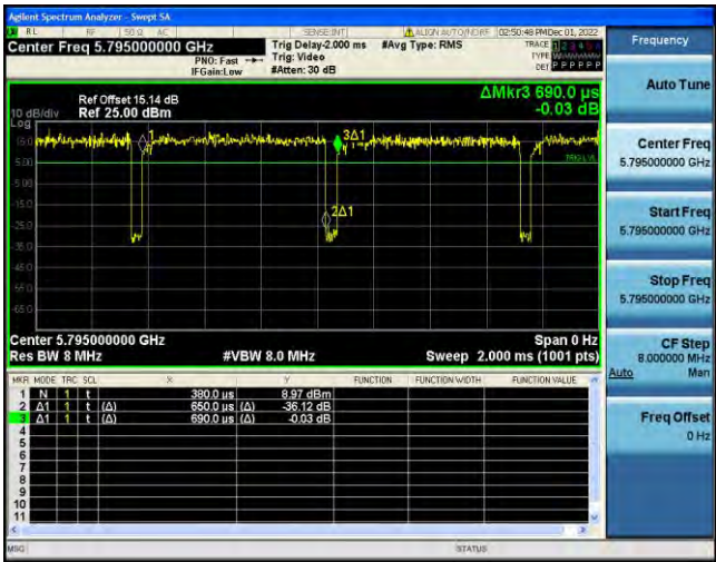
NTNV-11N40SISO-Ant2-5795-0.65-0.69
