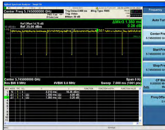
NTNV-11N20SISO-Ant2-5745-1.30-1.34
