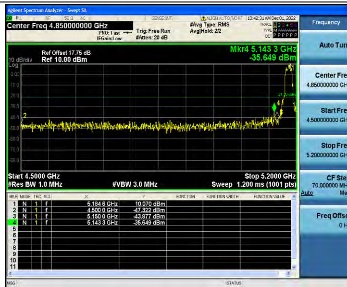
11A_Ant2_Low_5180_AV
