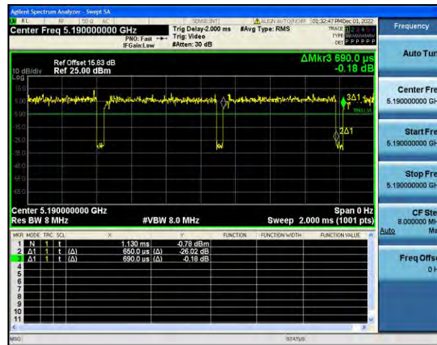
NTNV-11AC20SISO-Ant2-5180-1.32-1.36
