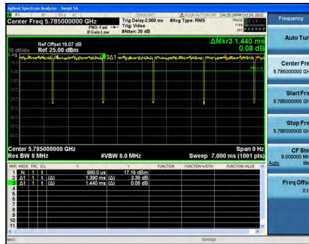
NTNV-11A-Ant2-5785-1.39-1.44
