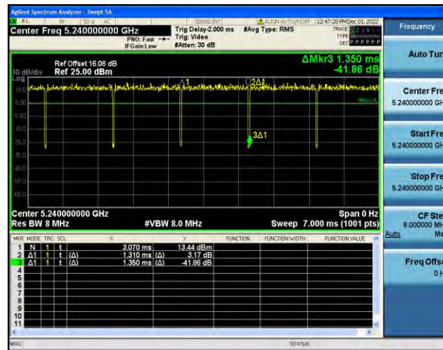
NTNV-11N20SISO-Ant2-5240-1.31-1.35
