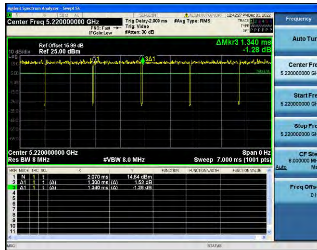
NTNV-11N20SISO-Ant2-5220-1.31-1.35
