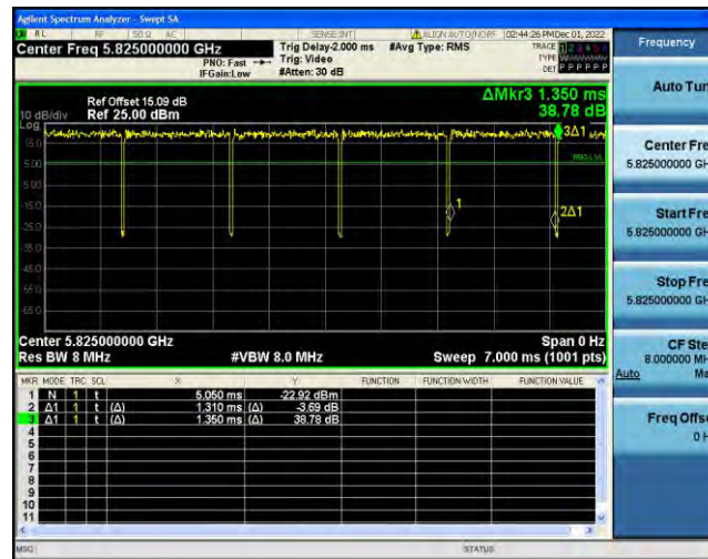
NTNV-11N20SISO-Ant2-5825-1.31-1.35
