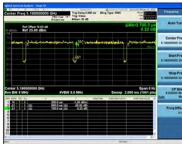
NTNV-11AC40SISO-Ant2-5190-0.66-0.70
