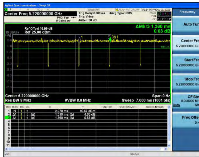
NTNV-11AC20SISO-Ant2-5220-1.32-1.36
