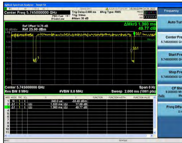
NTNV-11AC20SISO-Ant2-5745-1.31-1.36
