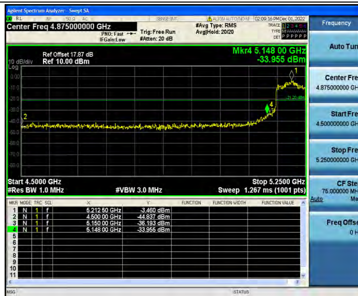
11AC80SISO_Ant2_Low_5210_AV
