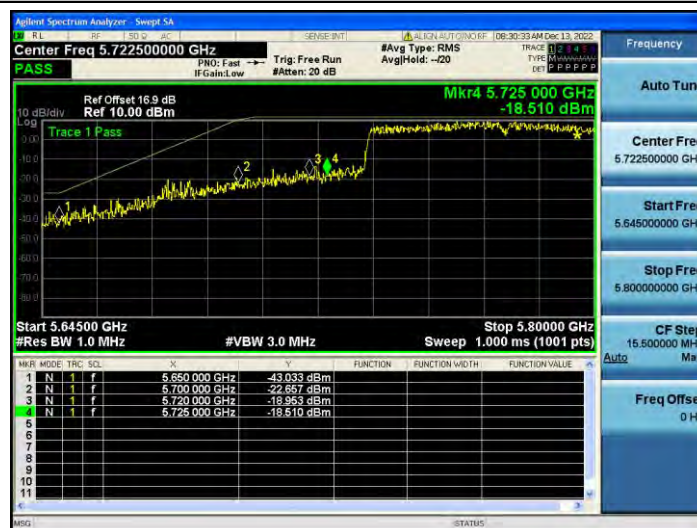
11AC80SISO_Ant2_Low_5775_Peak
