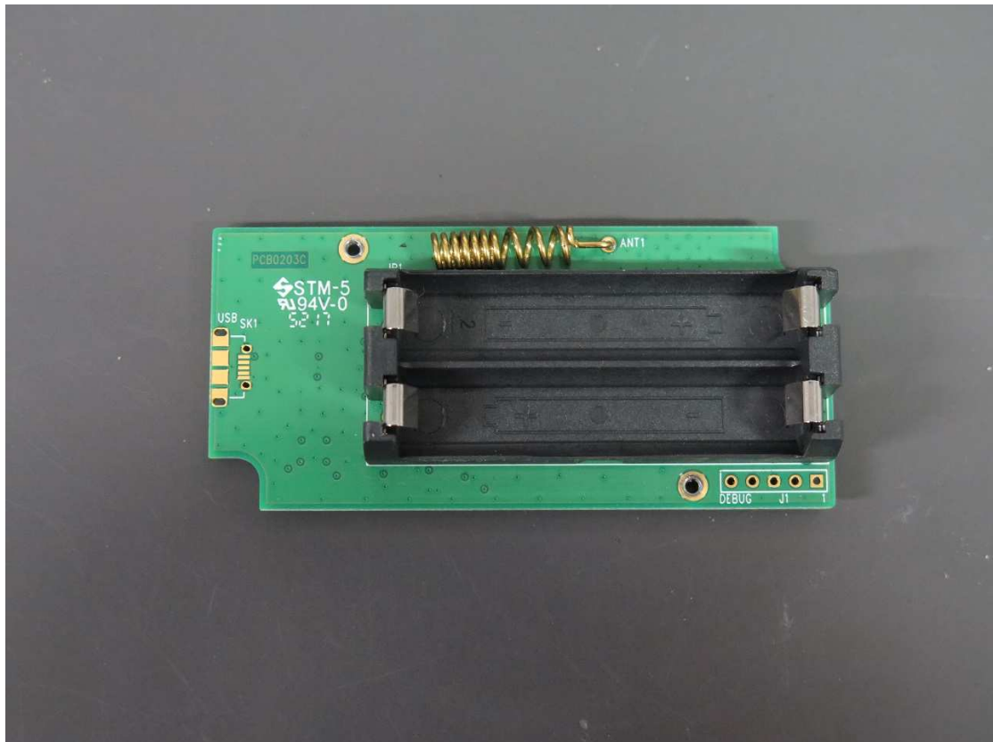
Motion Detection Sensor
