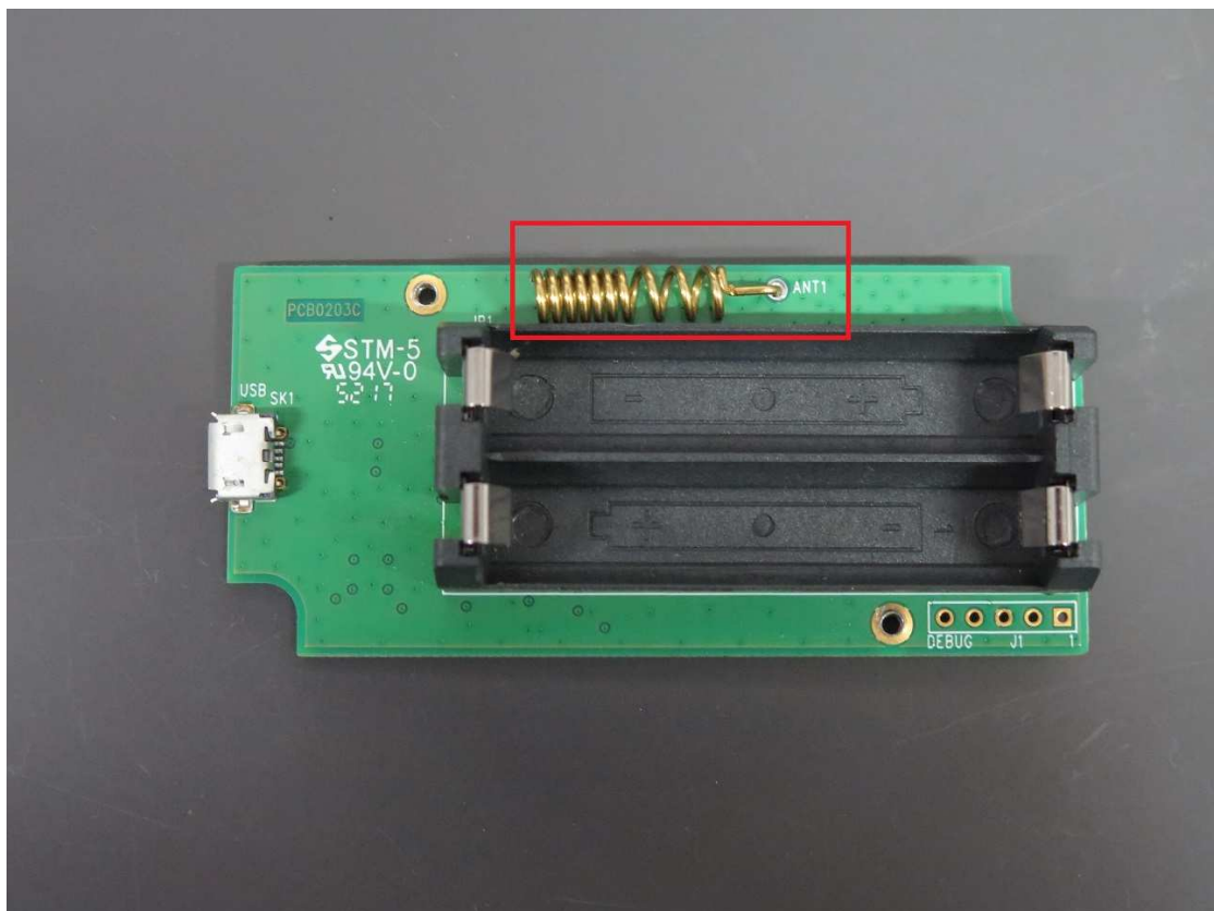
Shore Power Sensor (EUT antenna)
