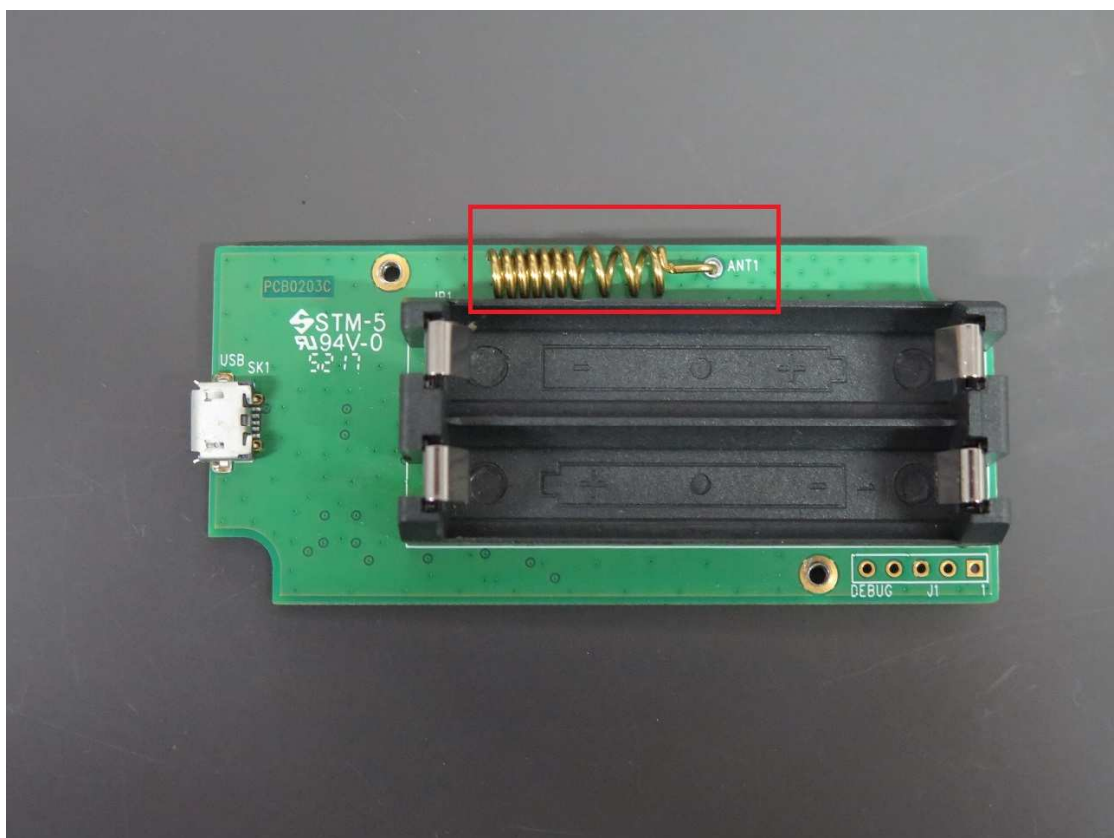
Temperature Sensor (EUT antenna)
