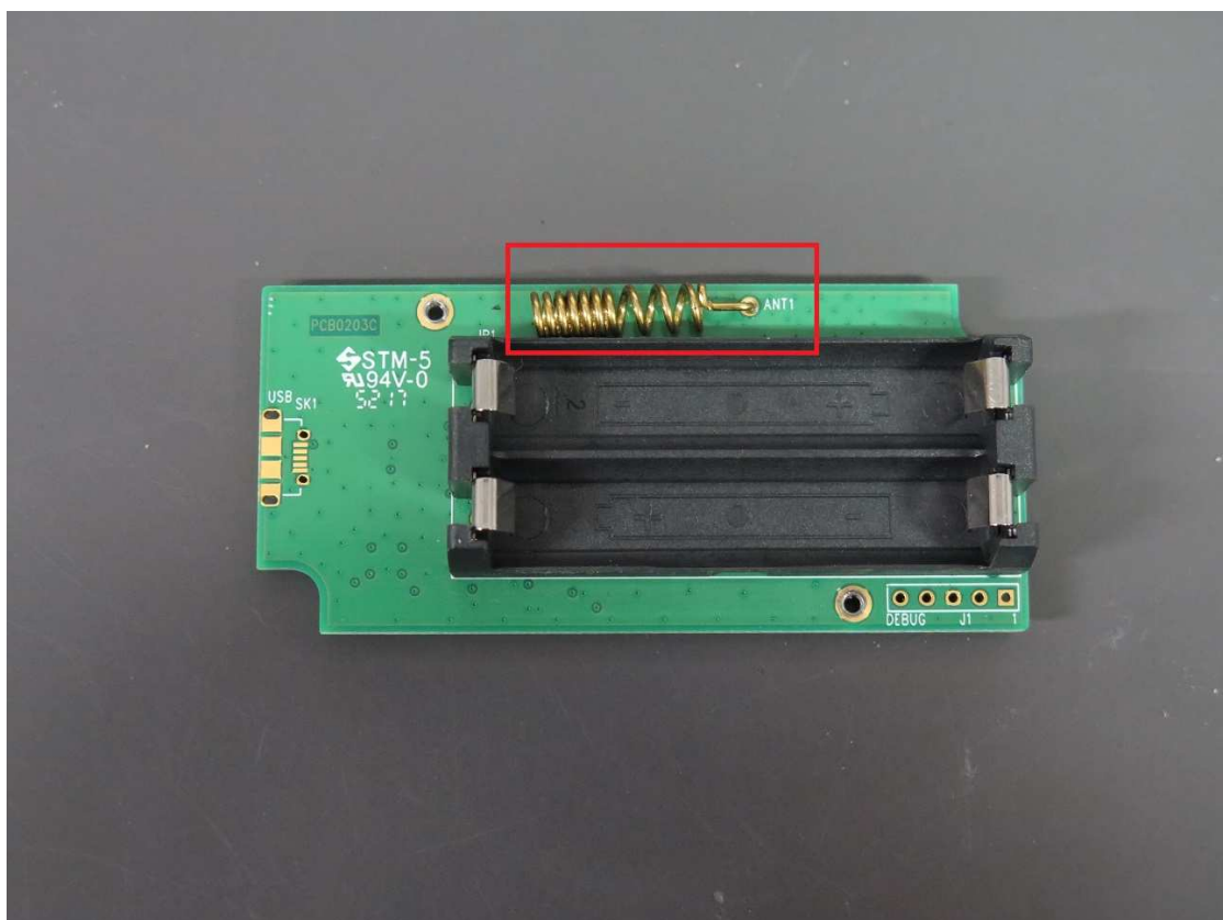
Motion Detection Sensor (EUT antenna)
