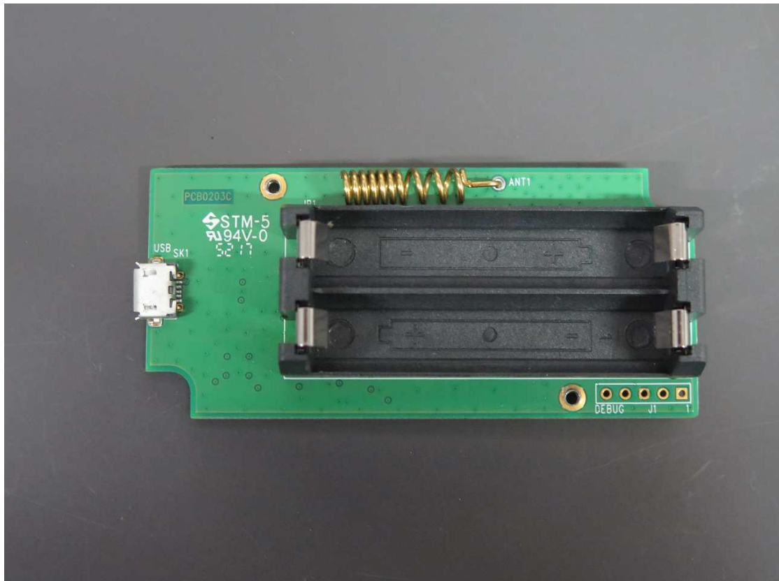
Temperature Sensor
