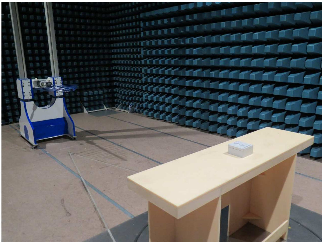
200Mz – 1GHz
