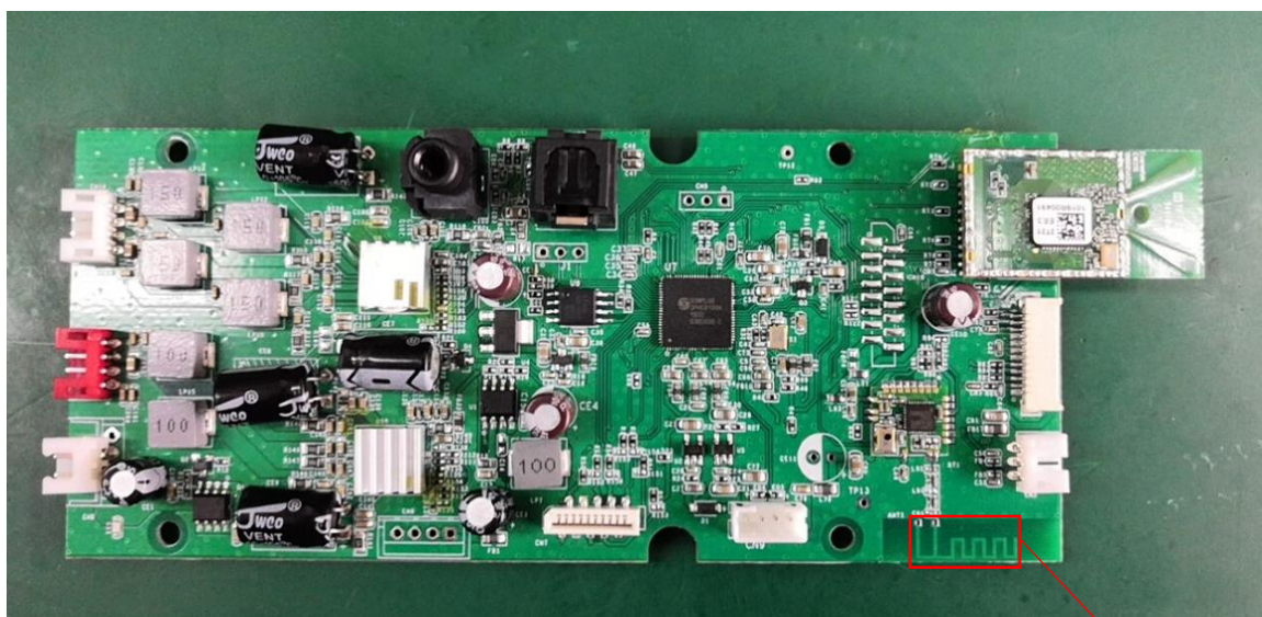
BT Antenna
