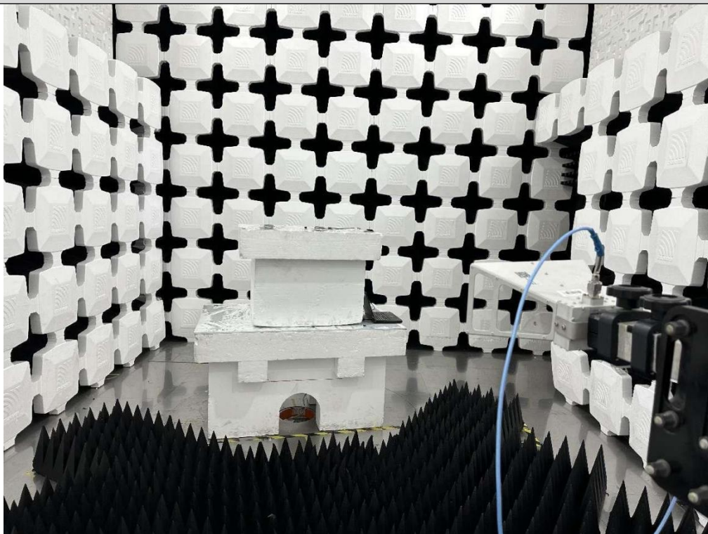
Conducted Test Setup Photograph
