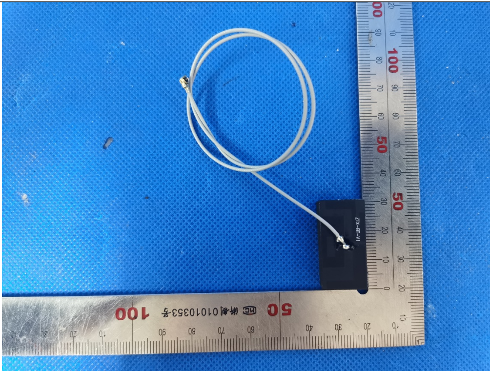
EUT Photo(6) 61005-00713
