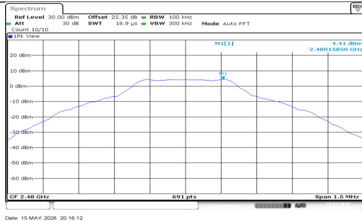
DH5_Ant2_2480_0~Reference
