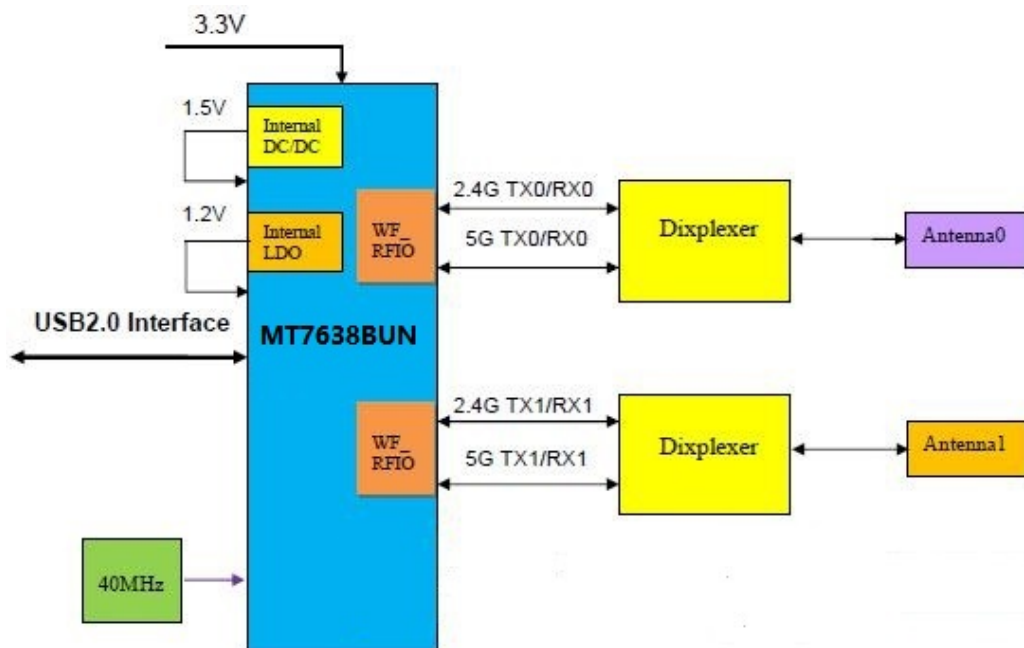
Figure 3.1 SKI.WB7638U.1_MT7638BU Block Diagram
