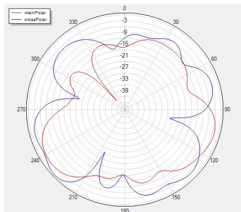
Phi=0 freq=5400MHz
