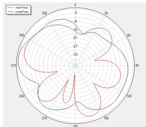
Phi=90 freq=5400MHz
