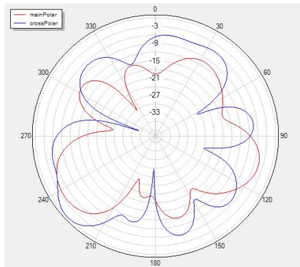
Phi=0 freq=5100MHz
