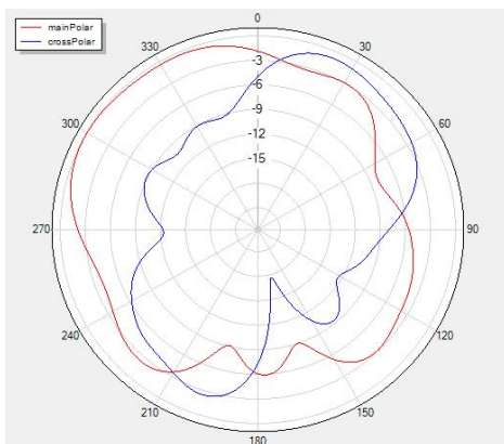
Phi=90 freq=2400MHz
