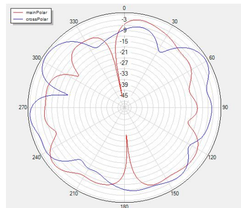
Theta=90 freq=5400MHz
