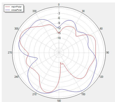
\Phi=90 freq=5900MHz
