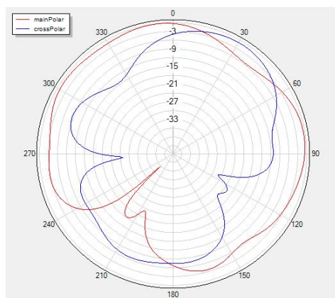
Phi=0 freq=2450MHz
