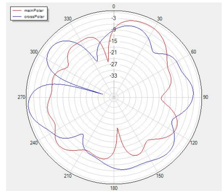
Theta=90 freq=5100MHz
