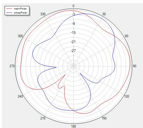
Phi=0 freq=2480MHz
