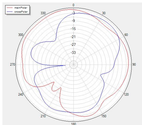
Phi=0 freq=2400MHz
