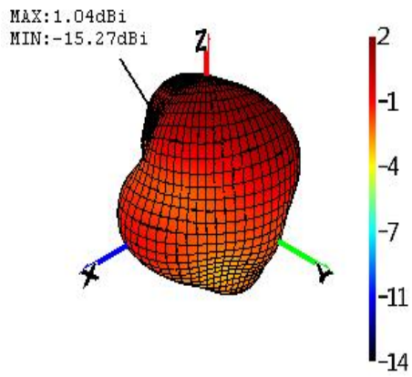
Phi=90 freq=5100MHz
