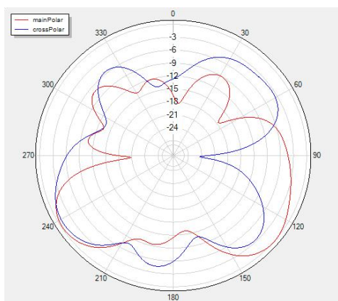
\Phi=0 freq=5900MHz
