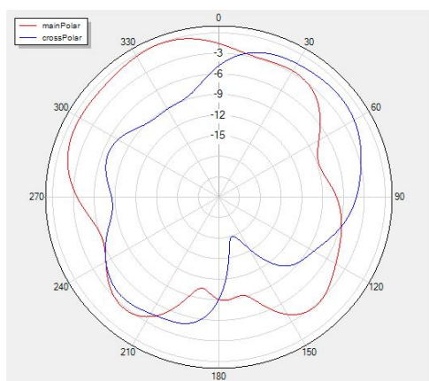
Phi=90 freq=2480MHz
