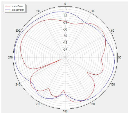
Phi=90 freq=5100MHz
