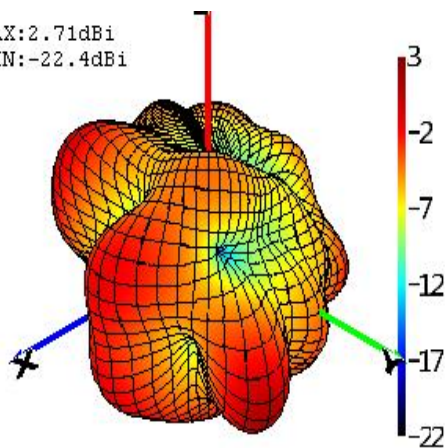
\Phi=90 freq=5900MHz
