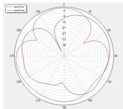
Theta=90 freq=2450MHz
