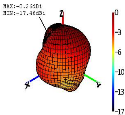
Phi=90 freq=2480MHz
