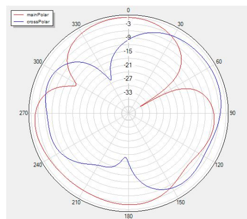
Theta=90 freq=2480MHz
