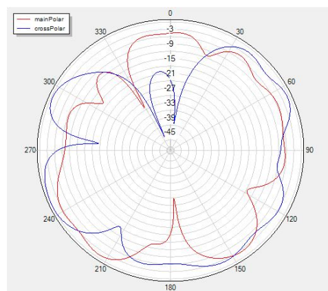
Theta=90 freq=5900MHz
