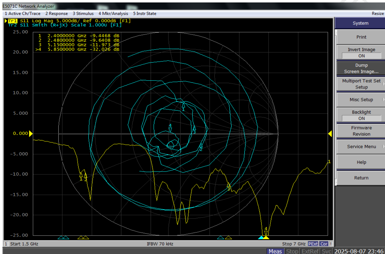
➤ Antenna S11 parameter diagram (WIFI 1 Antenna)
