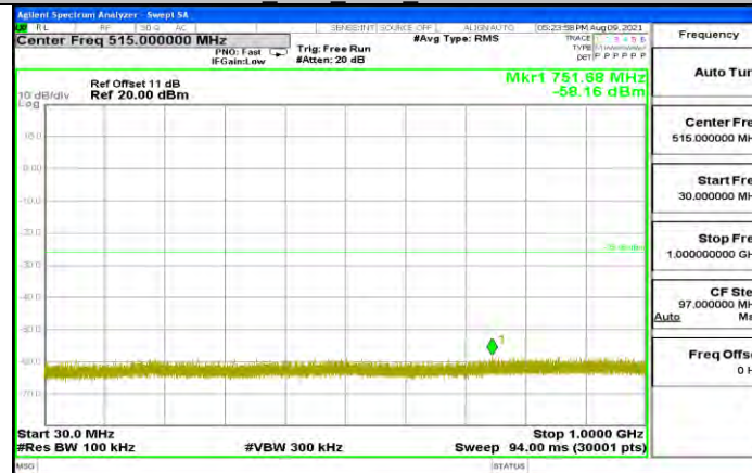
11G Ant1_2412_30~1000
