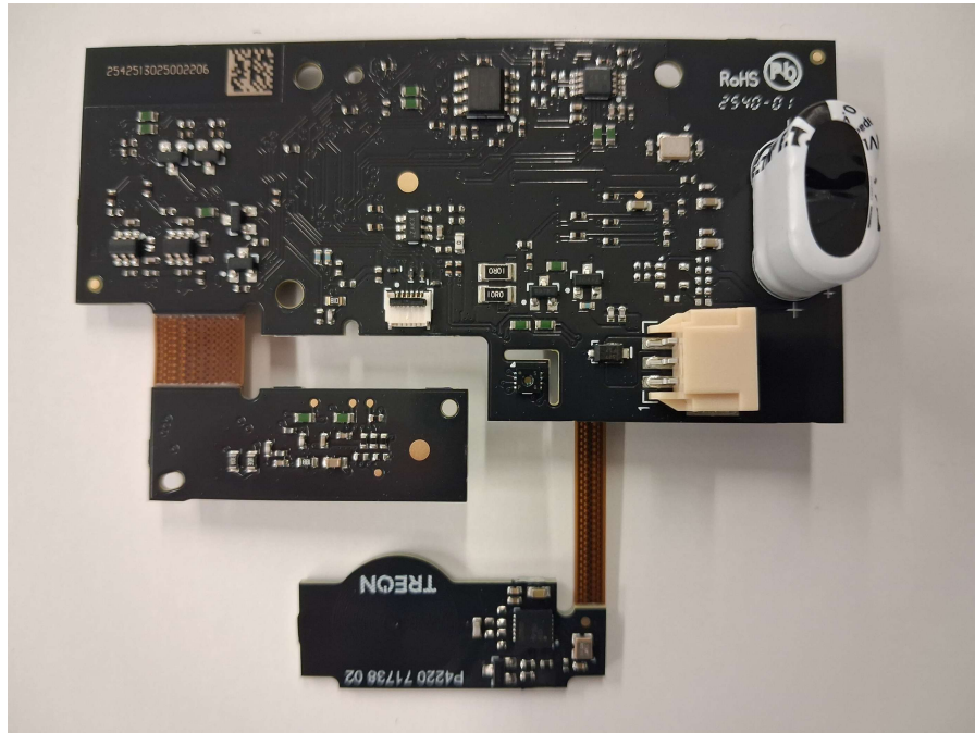
Picture 2. Main PCB, bottom view.
