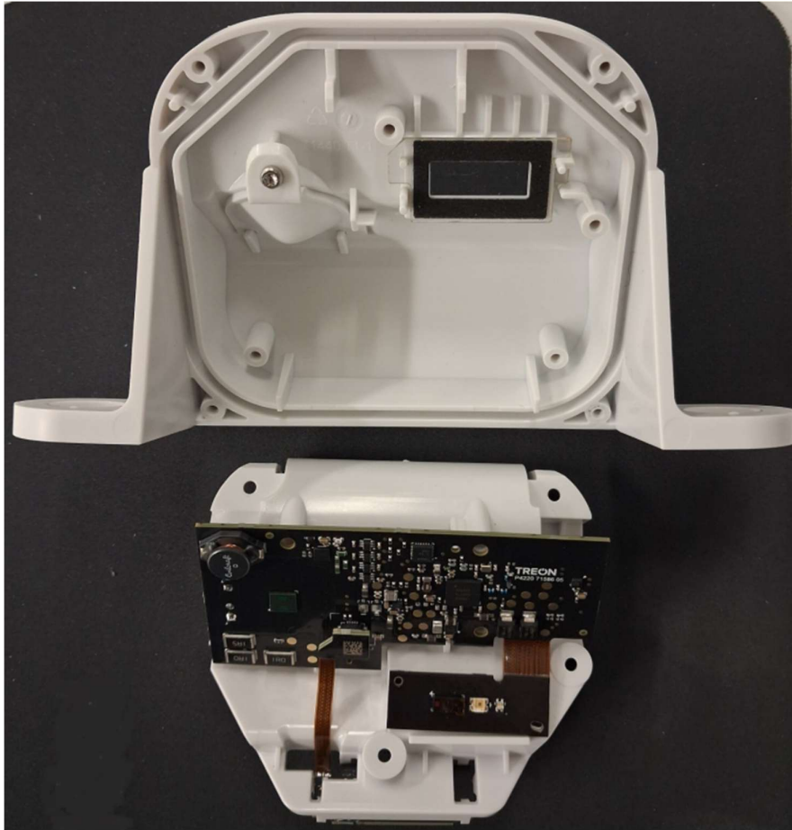
Picture 6. Main PCB location in the housing.
