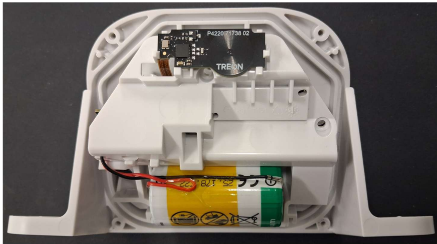
Picture 5. Coil PCB location in the housing.
