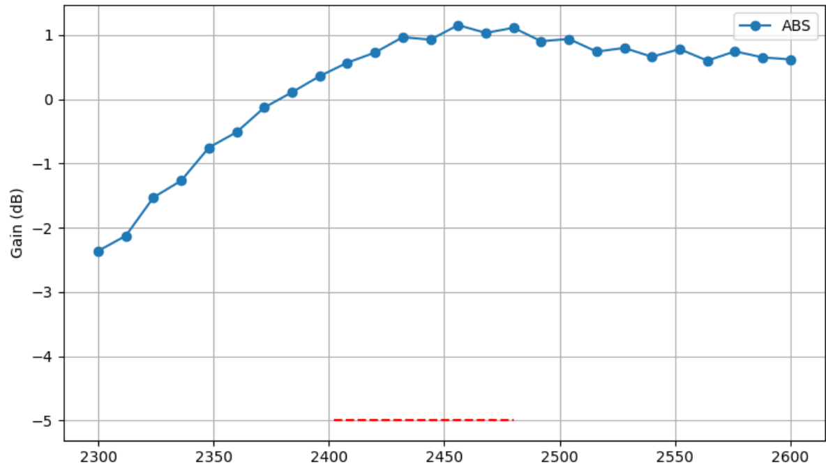
Figure 6 Antenna maximum gain vs. frequency
