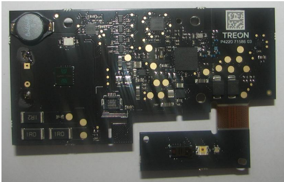
Figure 1 Product PCBA with integrated antenna. Antenna on the upper right corner
