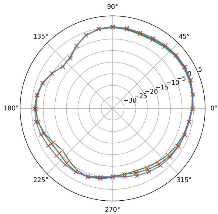
Figure 5 Antenna radiation pattern at 2408MHz, 2440MHz and 2484MHz. Horizontal and vertical polarization are summed together to obtain total radiated power.
