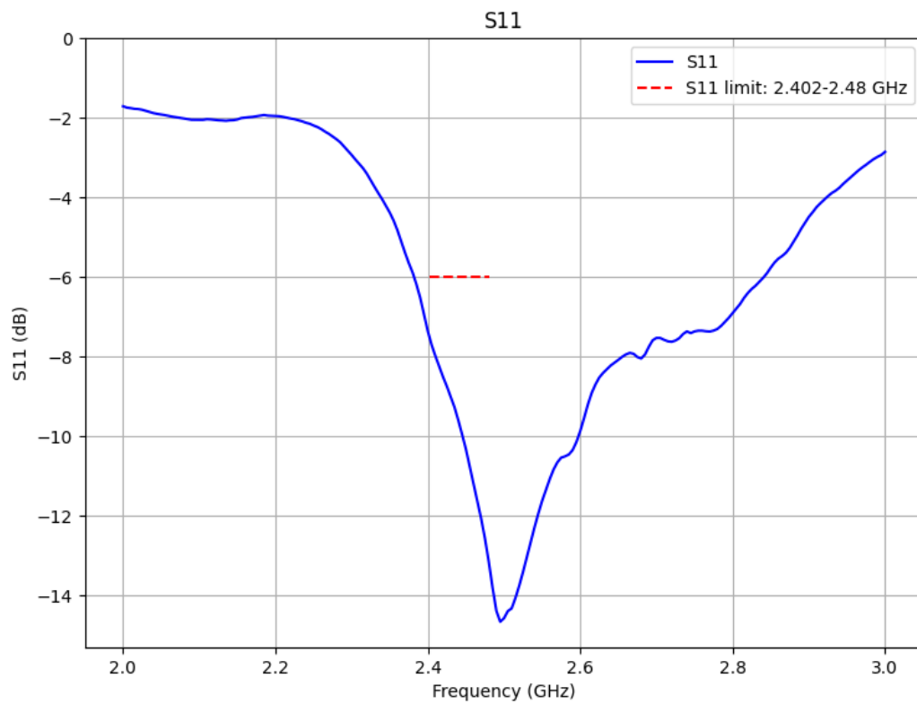
Figure 4 Antenna S_{11} in free space condition
