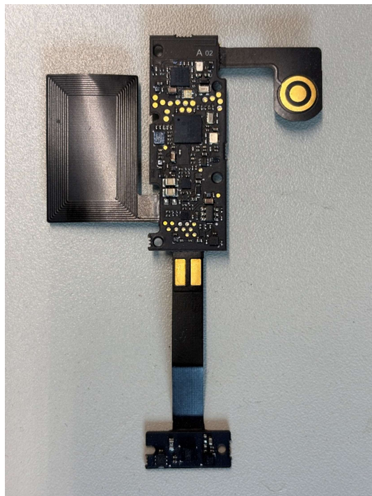
Picture 4. Device 2211 PCB top view.
