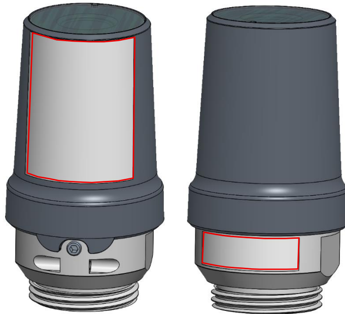
Picture(s) 1 and 2. Radio label area located on the device top cap and the device base. Label area marked with red rectangle.
