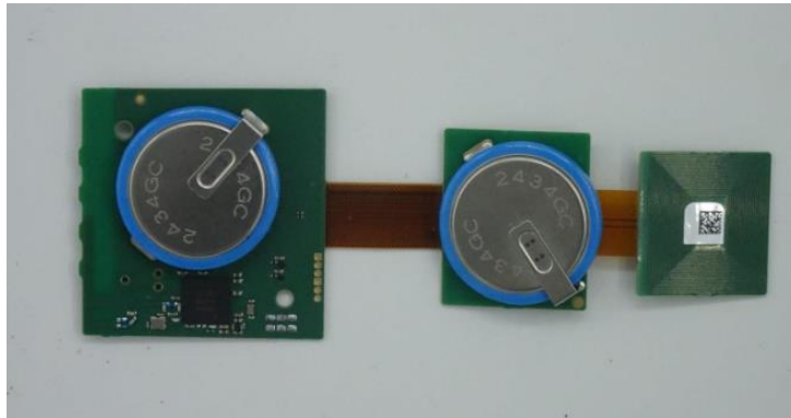
Picture 1. Device PCB top view.
