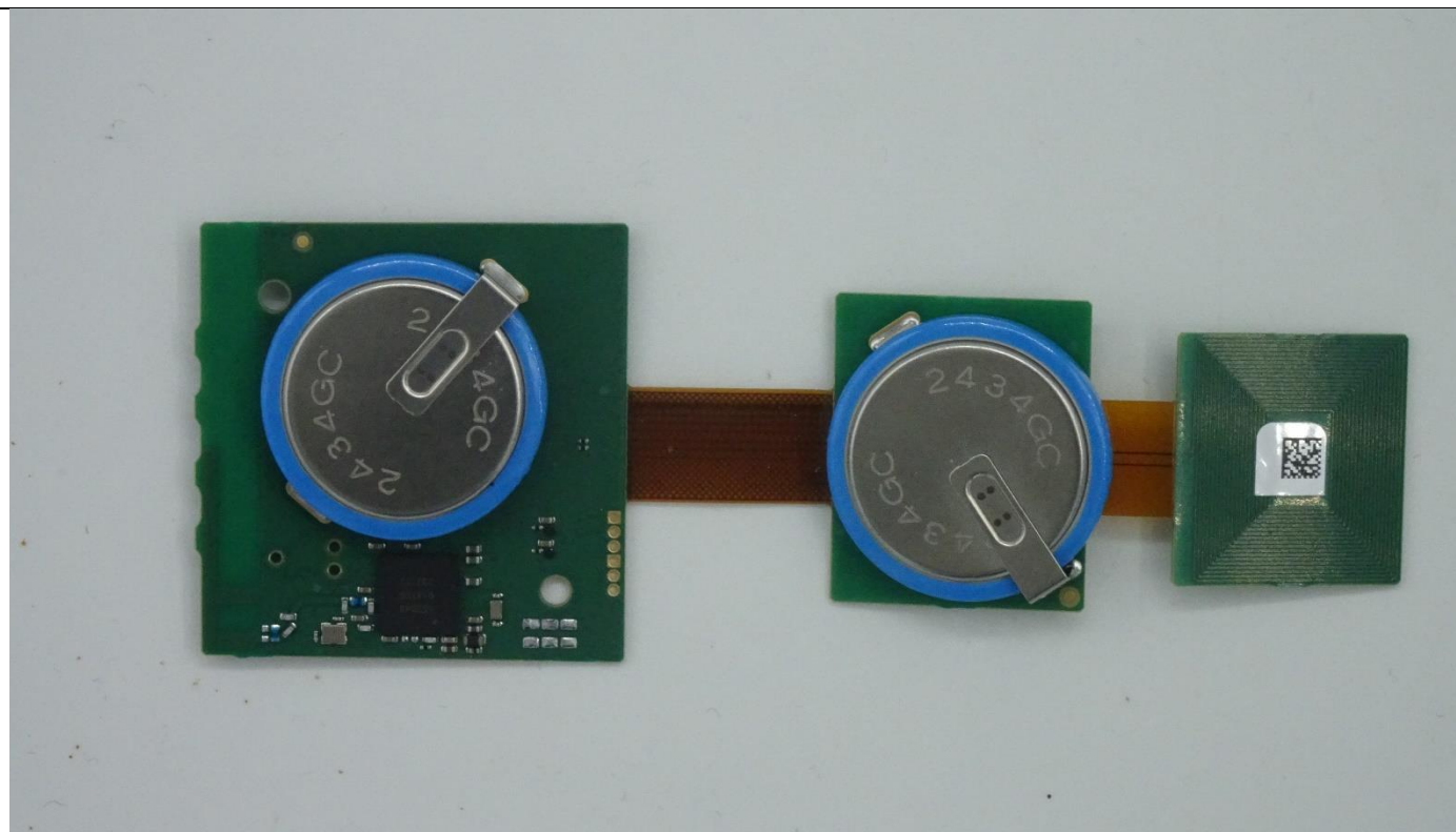
Picture 5, PCB top view
