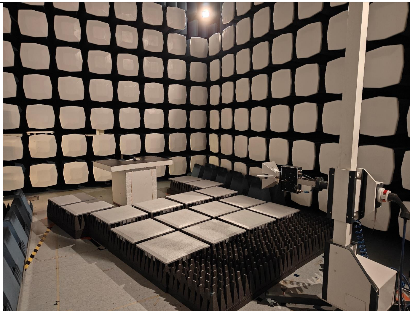
Picture 7, Radiated Emission, common setup, 1 – 12,75 GHz, front
