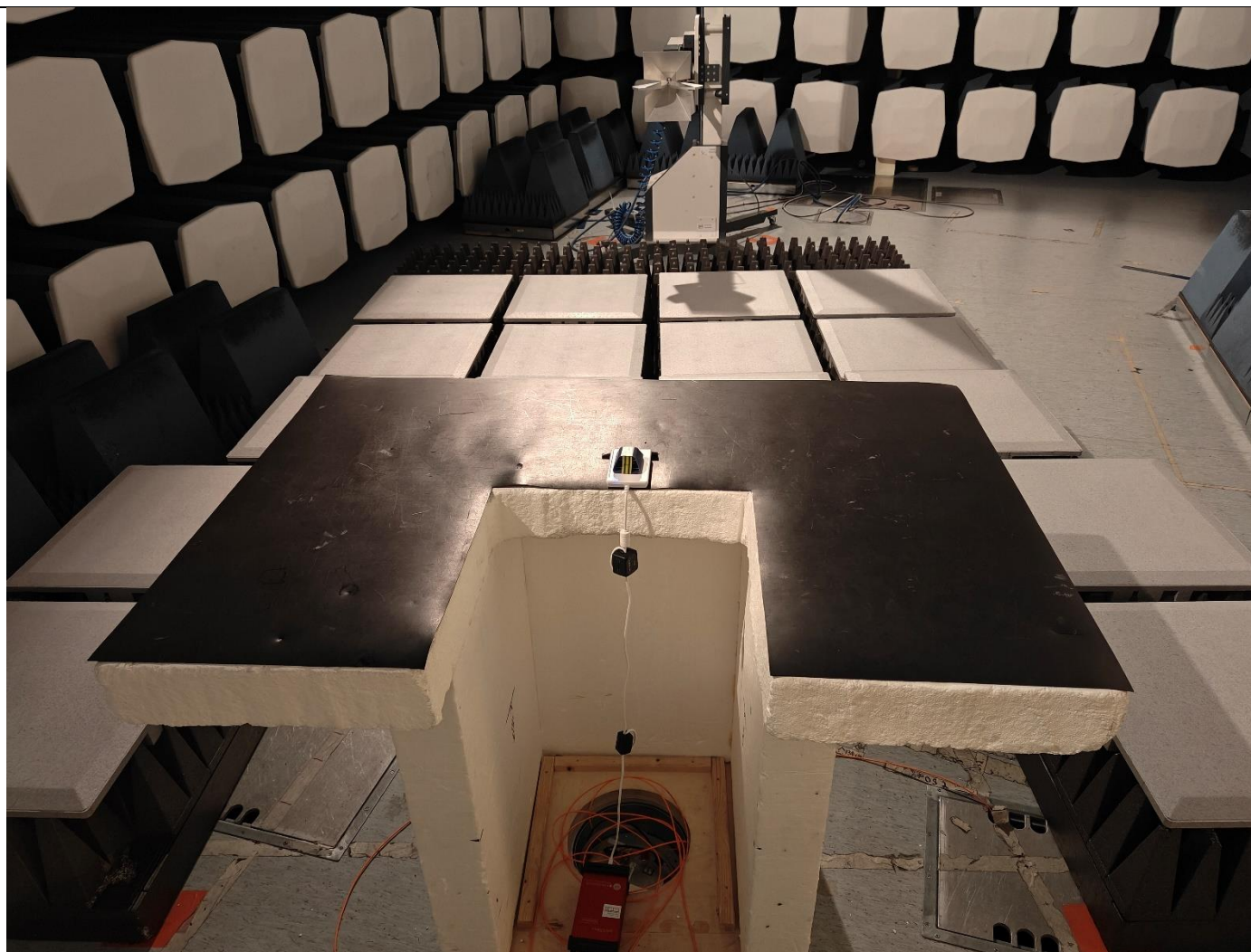
Picture 20, Radiated Emission, common setup, 1 – 12,75 MHz, back
