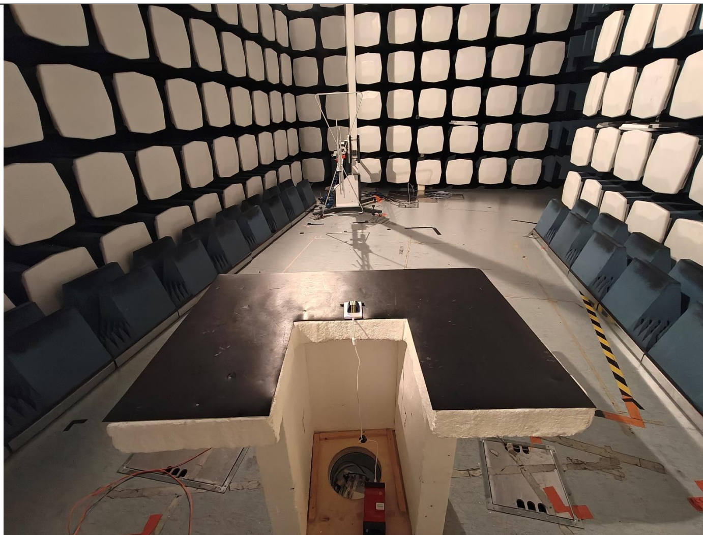
Picture 9, Radiated Emission, common setup, 30 – 1000 MHz, back
