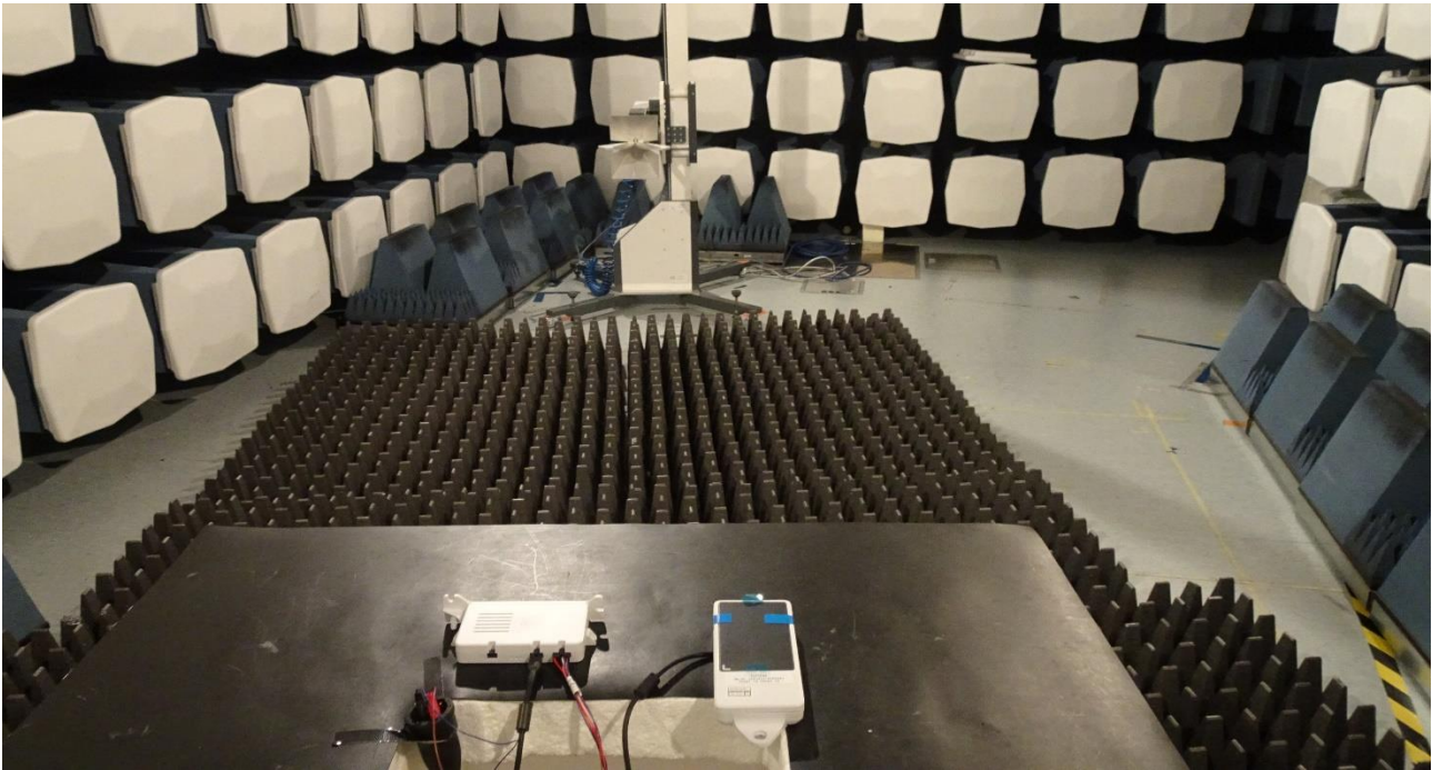
Picture 11 Radiated emissions, common setup 1 – 18 GHz, back
