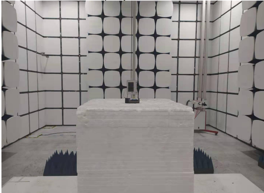
Radiated Spurious Emissions Test frequency from Above 1GHz
