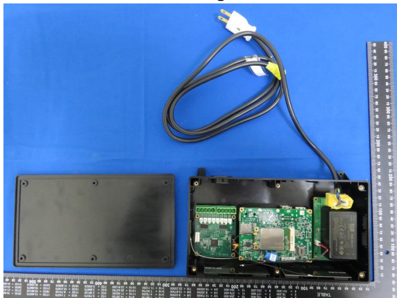
Dismantling View
