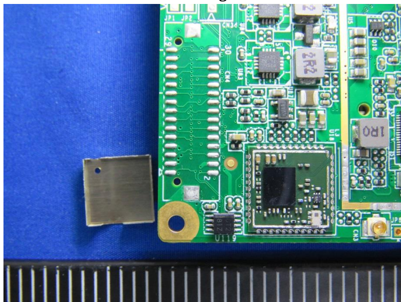
Dismantling View
