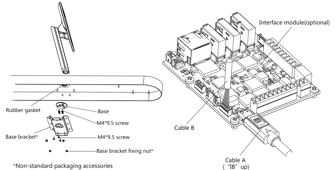
Installation diagram
