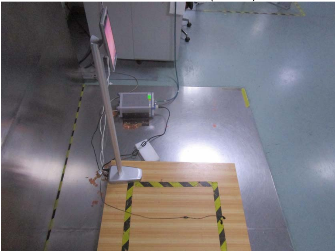
Conducted Emissions – Side View(AC Power)
