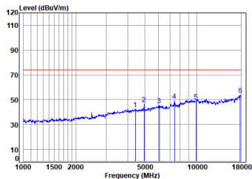
BLE_1M_TX_CH_39_Vertical-Peak
