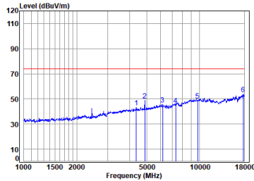
BLE_1M_TX_CH_20_Horizontal-Peak
