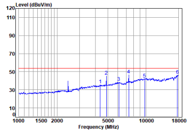
BLE_1M_TX_CH_20_Vertical-Avg
