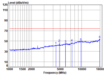
BLE_1M_TX_CH_20_Vertical-Peak
