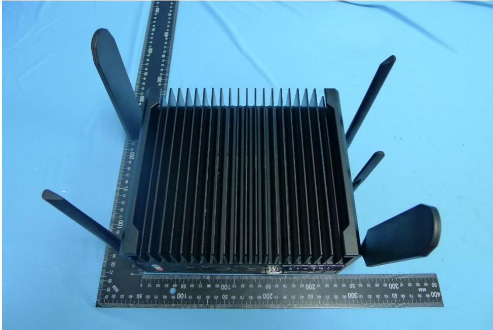
(1) EUT Photo
