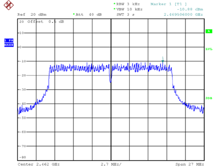
Mode: TX 11n HT20 2462MHz
