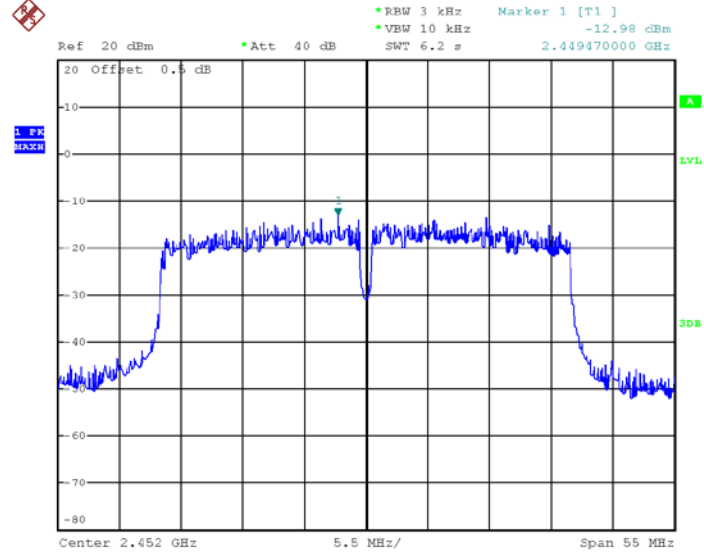
Mode: TX 11n HT40 2452MHz
