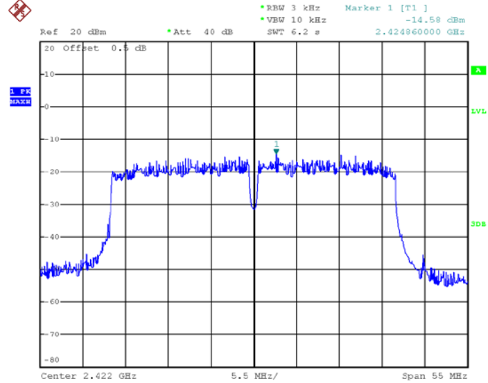
Mode: TX 11n HT40 2422MHz
