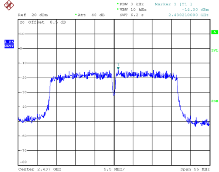
Mode: TX 11n HT40 2437MHz
