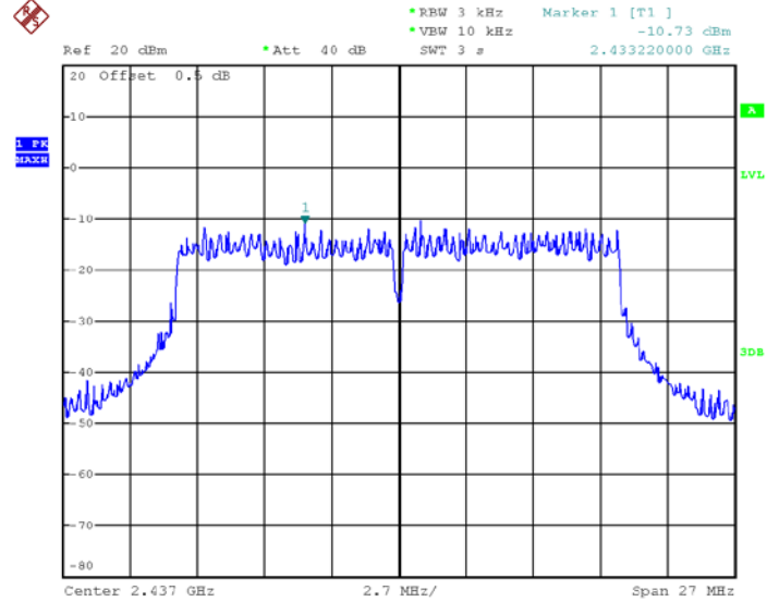
Mode: TX 11n HT20 2437MHz
