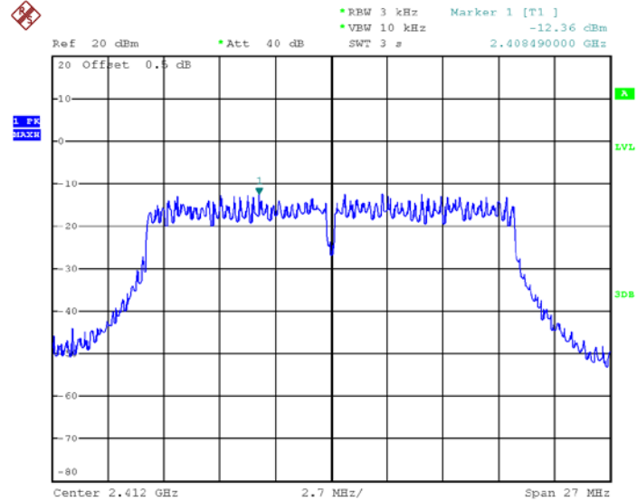
Mode: TX 11n HT20 2412MHz
