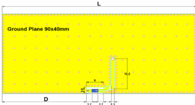
Antenna S11 on Type-1 Test Board
