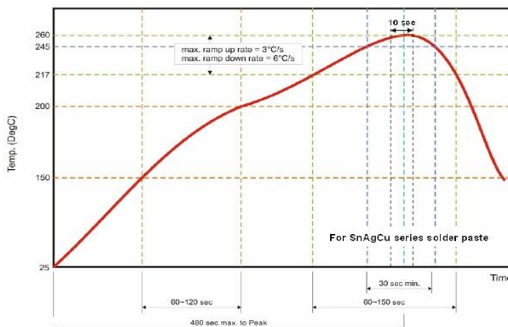
Fig 2. Infrared soldering profile
