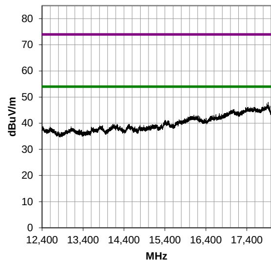
12400-18000 MHz, Run 5
