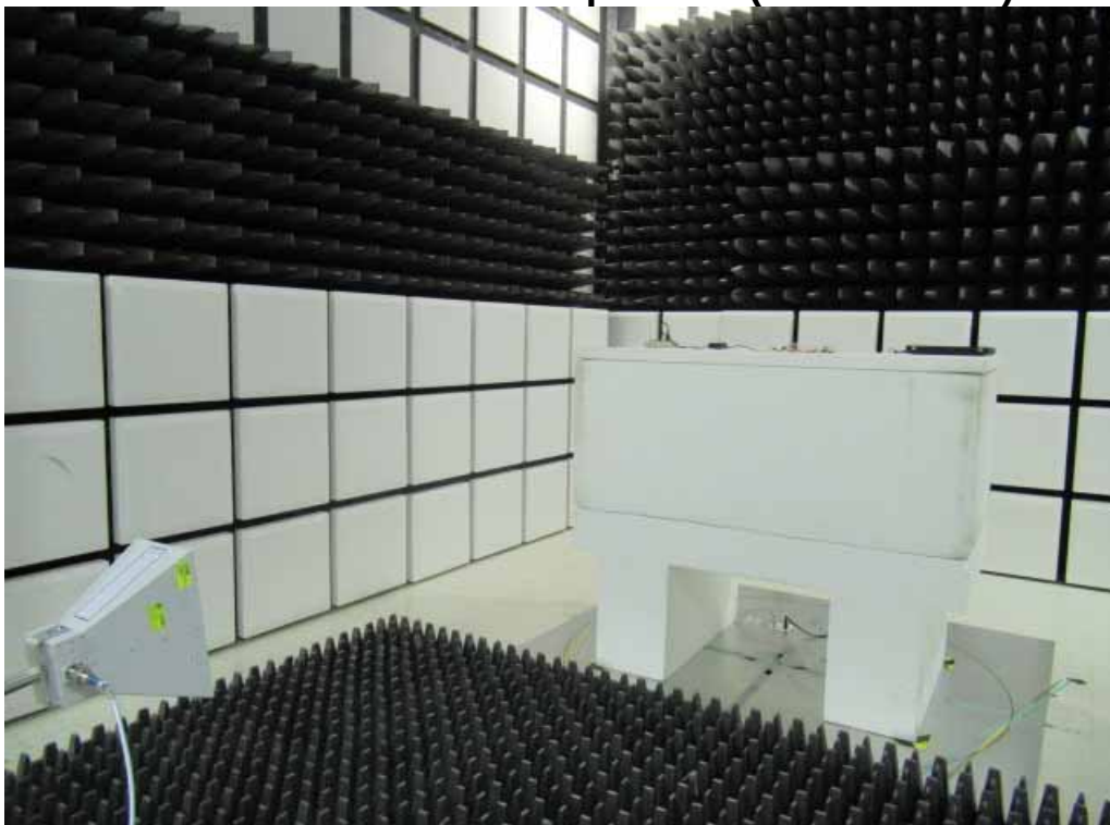
Radiated Emission Set up Photo (Front View)
