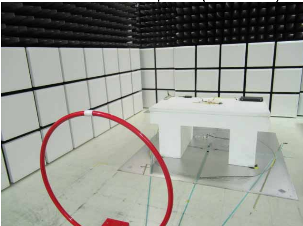
Radiated Emission Set up Photo (Below 1GHz)
