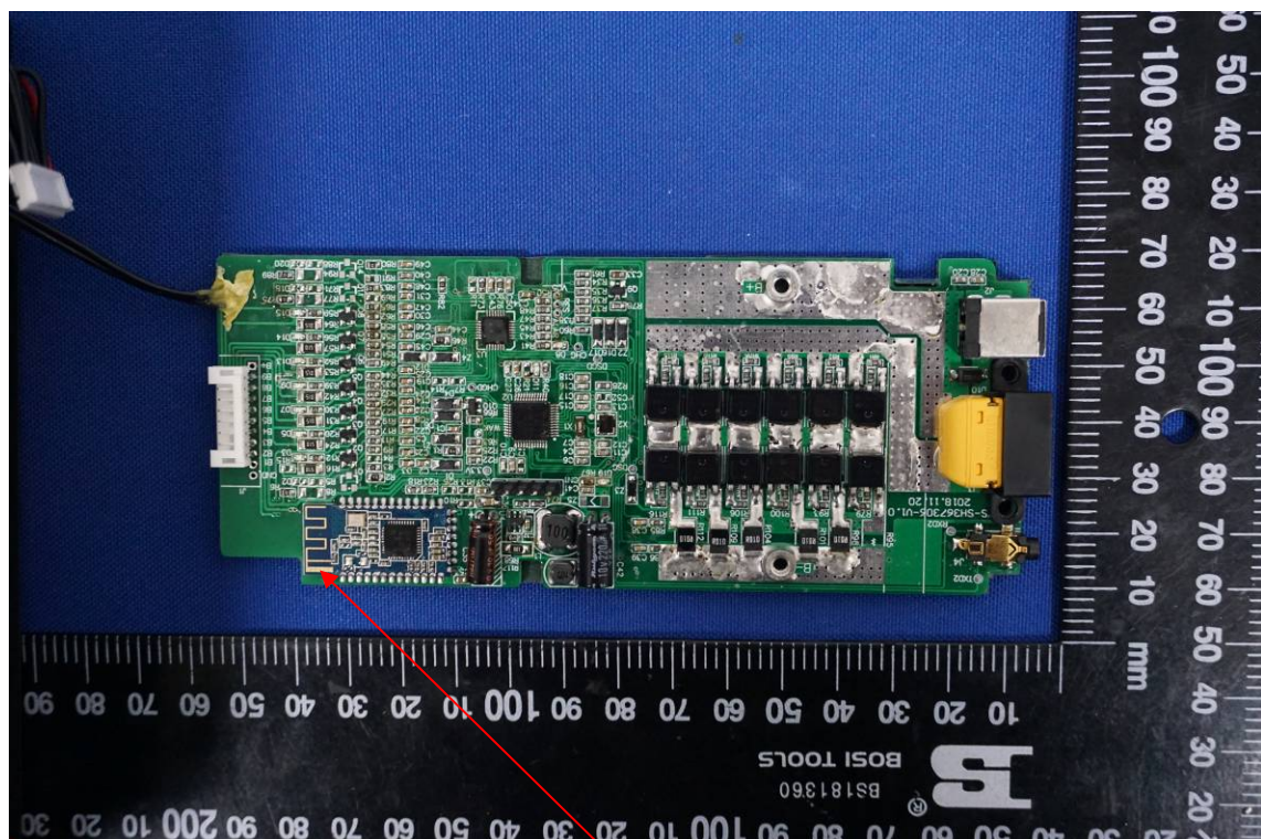
BT Antenna
