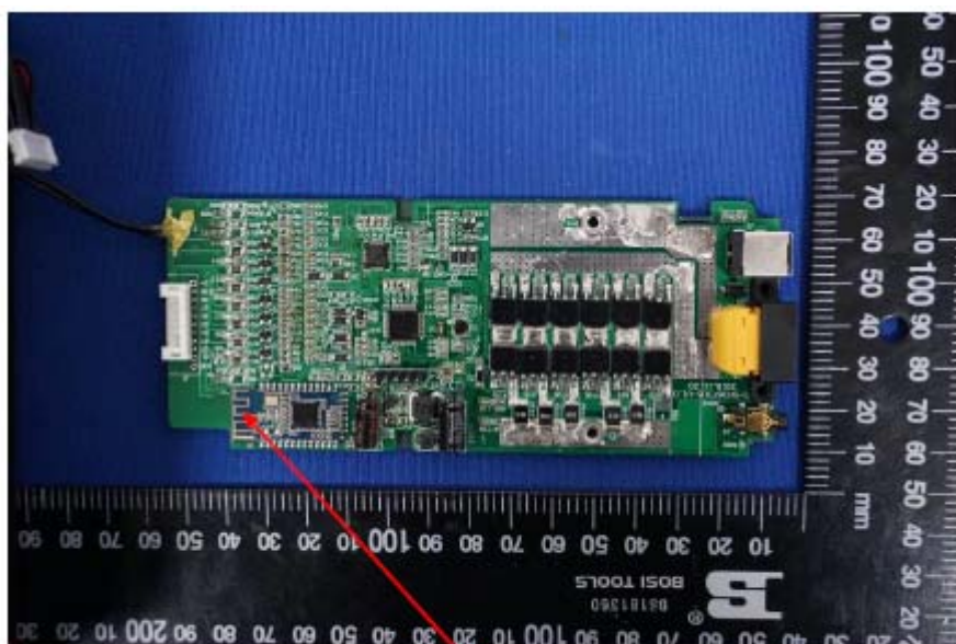
BT Antenna
