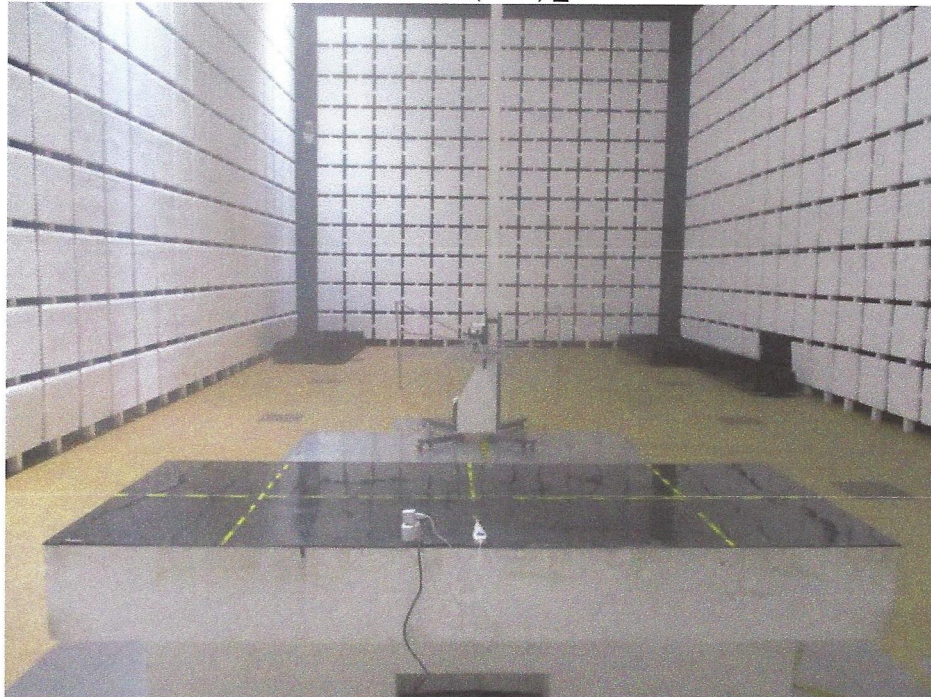
Radiated Emission (Rear)_Below 1 GHz
