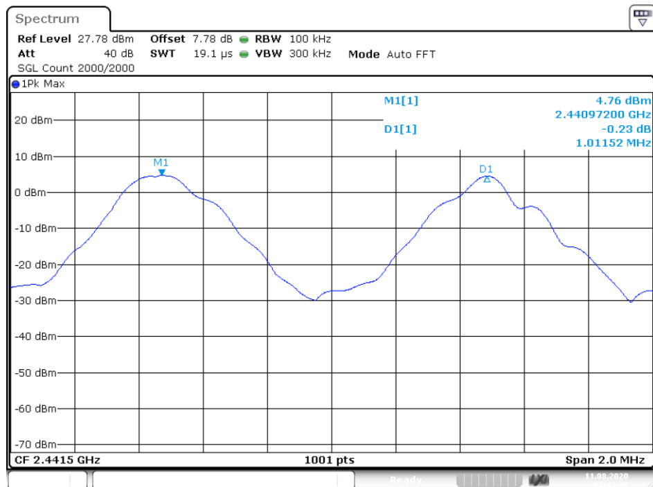
CFS NVNT user 2441MHz
