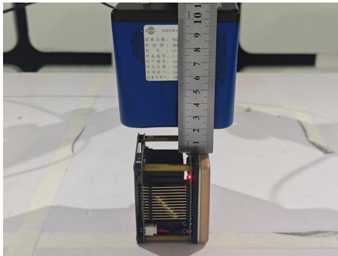
Right Side (Test distance: 2cm)
