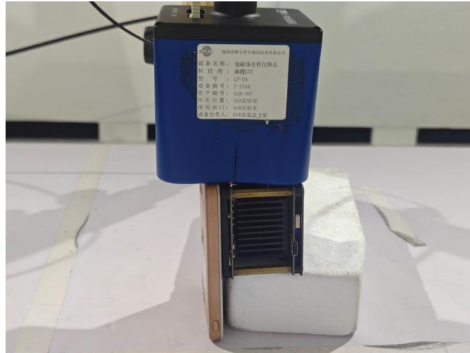
Top Side (Test distance: 0cm)
